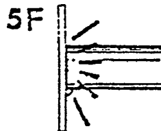
FIGURE 5. Fillet weld in tube: positions 1F, 2F, 4F, and 5F.
