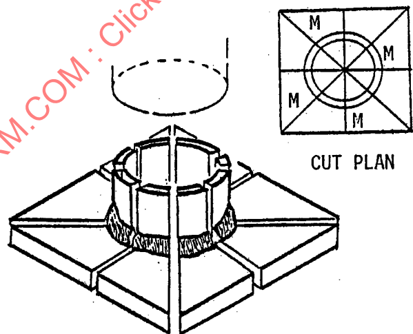
FIGURE 20. Blank locations for metallographic specimens in fillet-welded tube.
