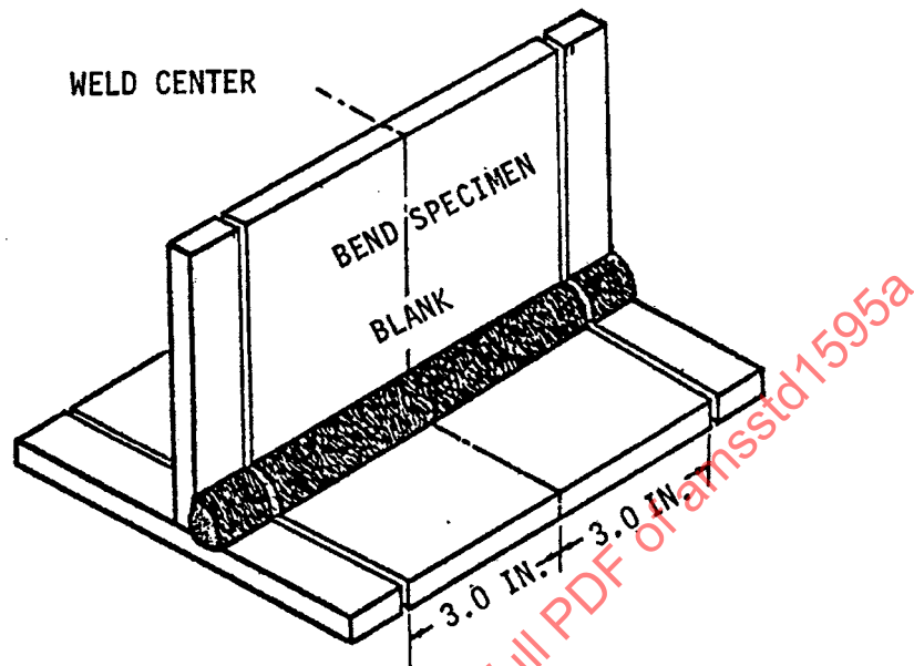
FIGURE 14. Blank location for bend specimens in fillet-welded sheet.
