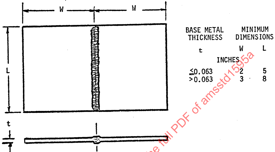
FIGURE 6. Groove test weld in sheet.
