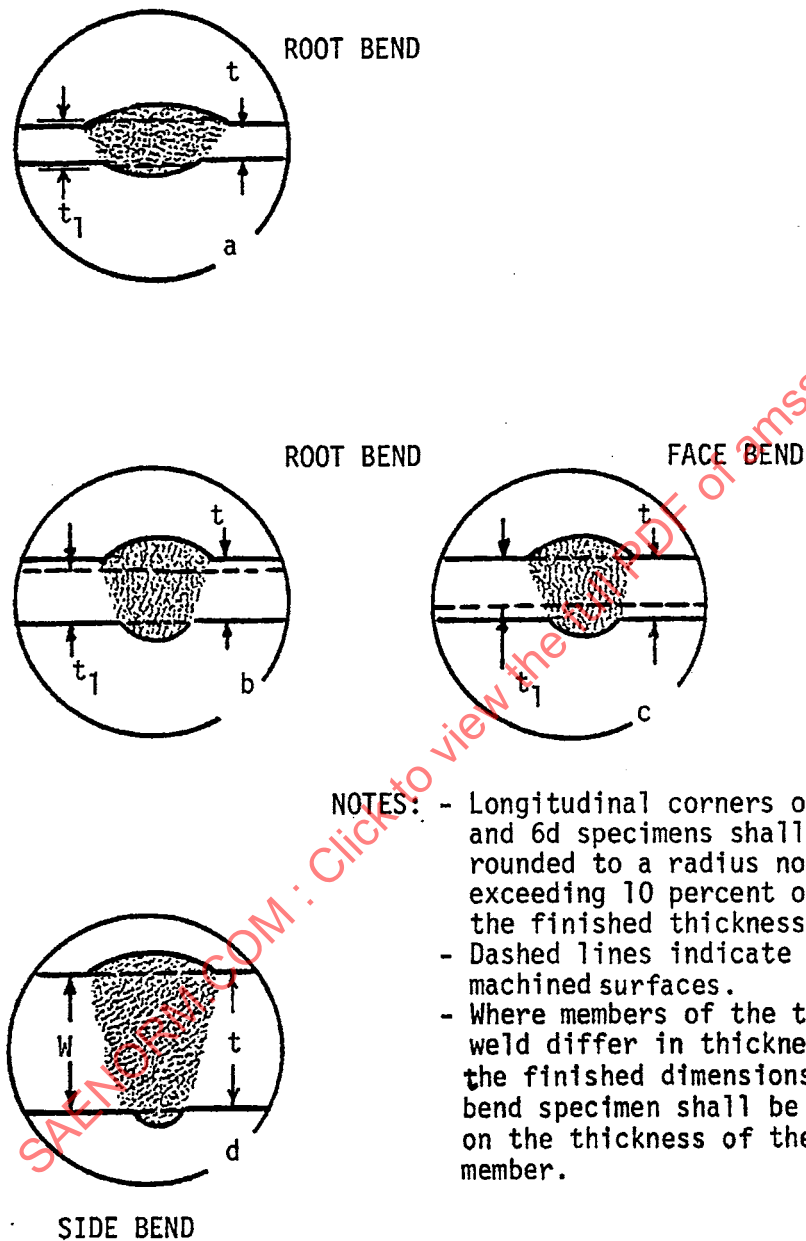
FIGURE 11. Bend specimens in groove-welded sheet. Continued.
