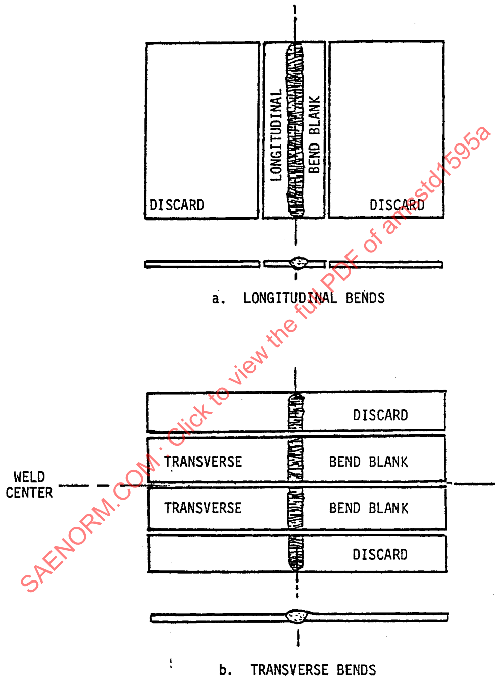
FIGURE 10. Blank locations for bend specimens in groove-welded sheet.
