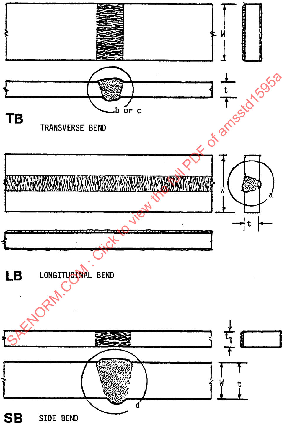
FIGURE 11. Bend specimens in groove-welded sheet.
