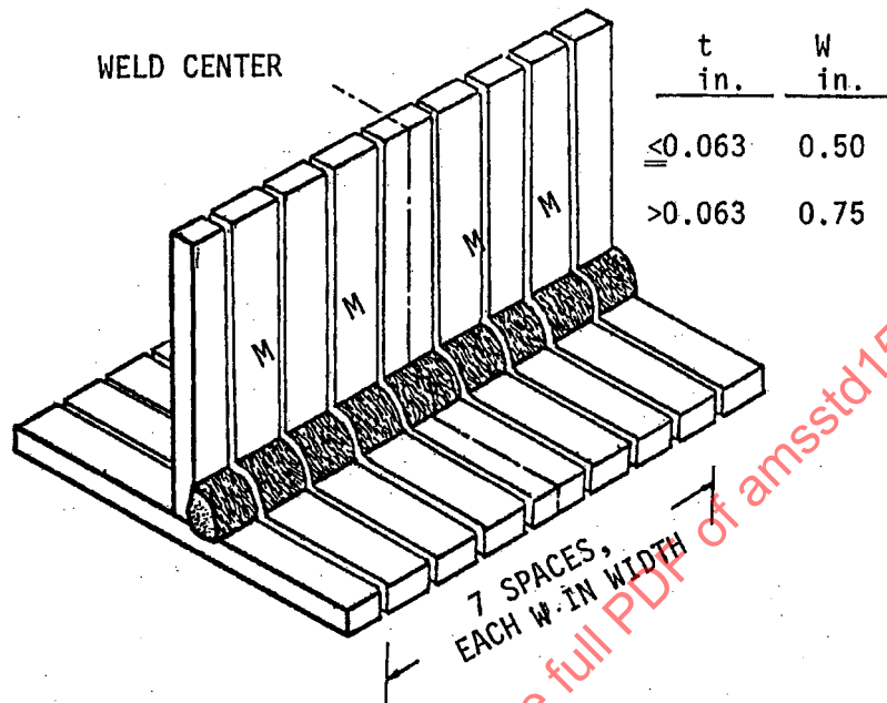
FIGURE 19. Blank locations for metallographic specimens in fillet-welded sheet.
