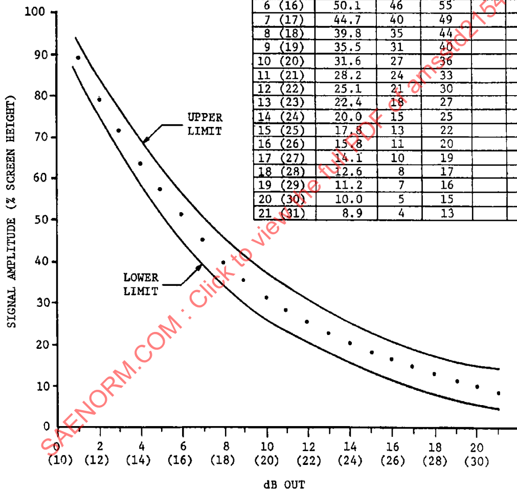
FIGURE 2 DB ATTENUATOR CHECK DATA SHEET
