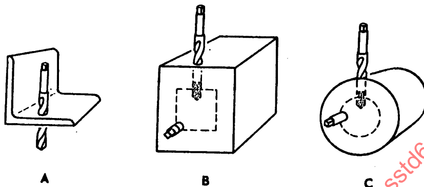
FIGURE 1. Drill locations for obtaining product analysis samples
