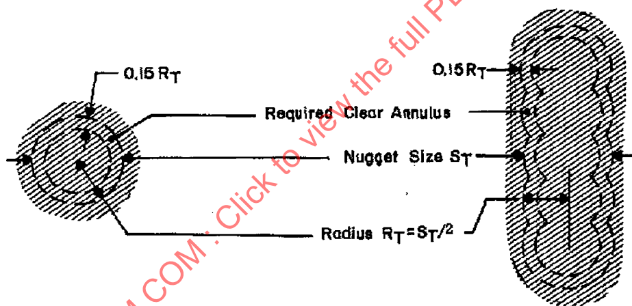
FIGURE 8. Nomenclature diagram of spot and seam weld radiographs
