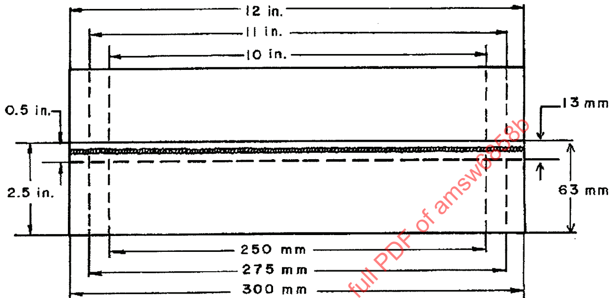
Figure 6a. Seam weld specimen.
