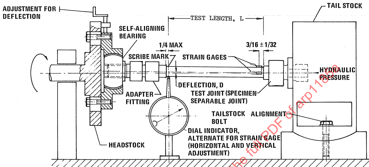
FIGURE 1 - ROTARY FLEXURE TEST SCHEMATIC
