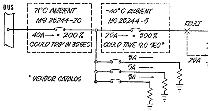
FIGURE 5.c COORDINATION MISAPPLICATION (Same Family - Different Ambient)
