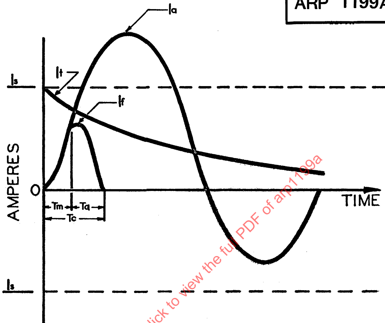
FIGURE 6.b TYPICAL CURRENT-LIMITING FUSE LET-THRU CURRENT CURVE AND PROSPECTIVE FAULT CURRENT CURVE.
