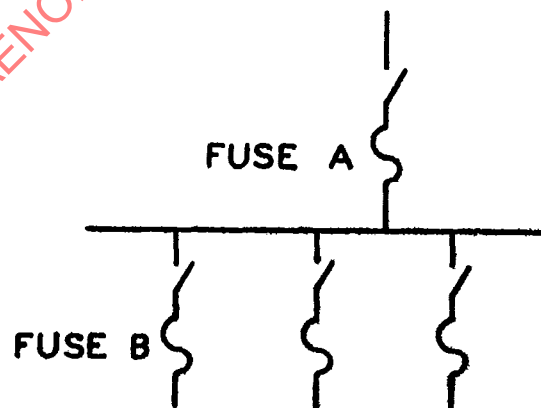
FIGURE 6.g Coordination of fuses A & B. A fault on the load side of fuse B will be isolated by fuse B without disturbing fuse A.
