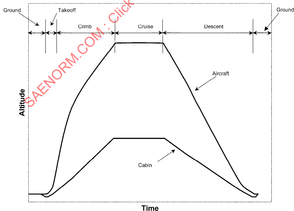
FIGURE 7 - CABIN PRESSURE SCHEDULE FOR A TYPICAL COMMERCIAL AIRCRAFT
