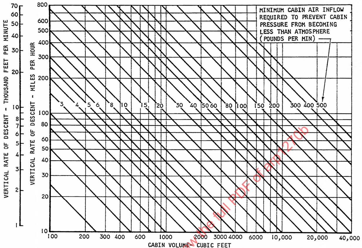
FIGURE 8 - MINIMUM CABIN AIR INFLOW REQUIRED TO PREVENT CABIN PRESSURE FROM BECOMING LESS THAN AMBIENT
