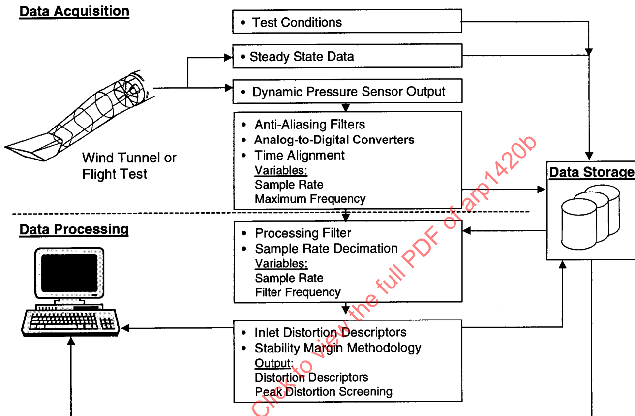
FIGURE 3- Digital Data Acquisition, Processing and Storage
