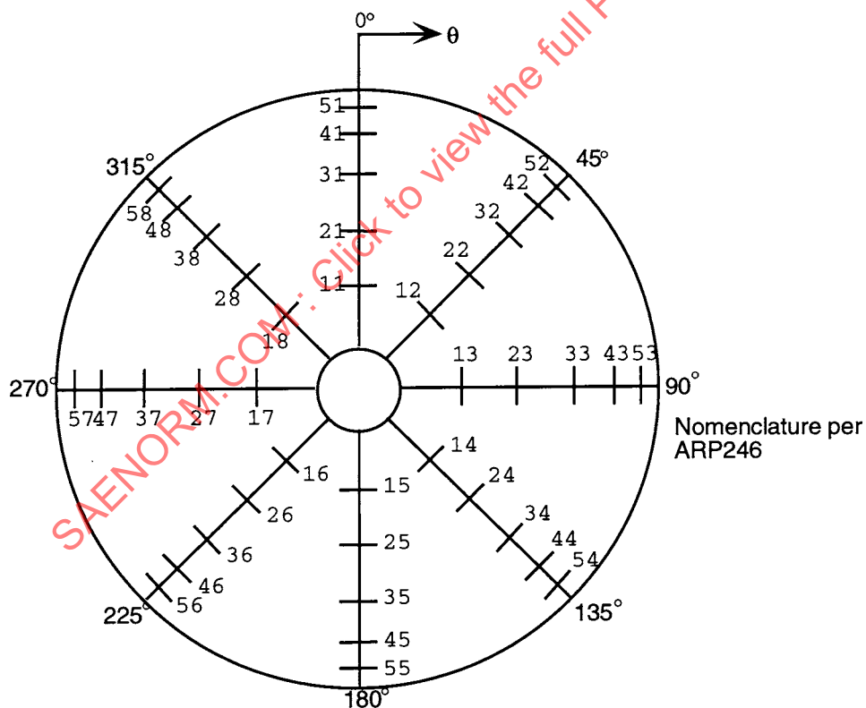
FIGURE 2 - Probe Orientation - View Looking Forward
