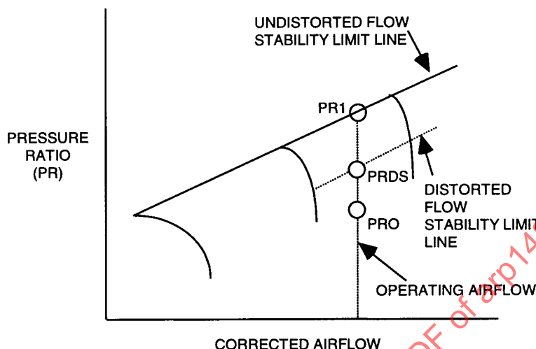
FIGURE 1 - Stability Margin Definition
