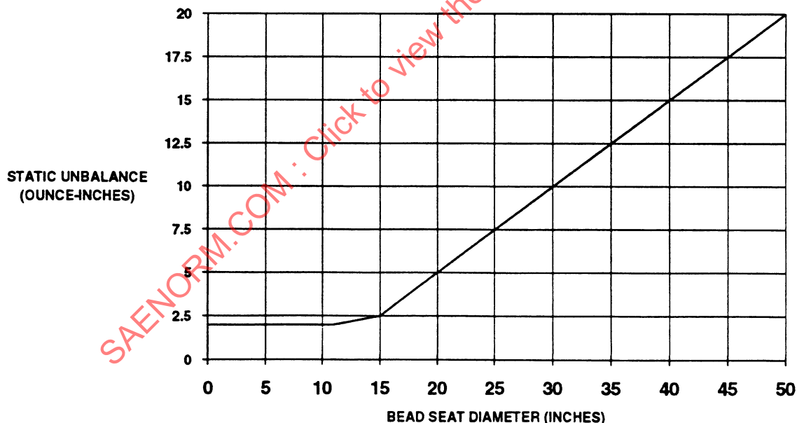
FIGURE 1 - Allowable Static Unbalance
