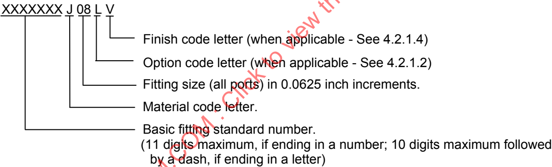
FIGURE 7 - PART NUMBER STRUCTURE FOR NOMINAL SIZE FITTINGS OR FITTING ASSEMBLIES OF ONE MATERIAL
