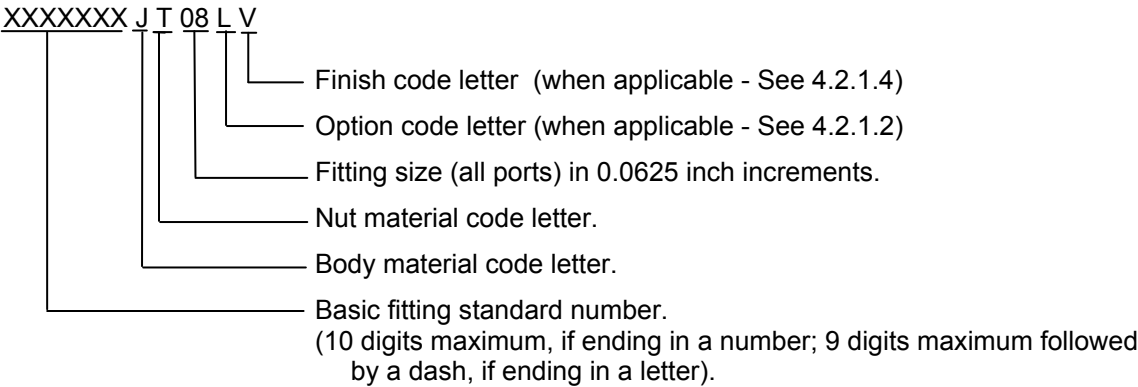
FIGURE 8 - PART NUMBER STRUCTURE FOR NOMINAL SIZE FITTING ASSEMBLIES OF DIFFERENT MATERIALS
