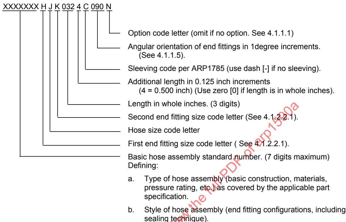
FIGURE 6 - 19 DIGIT PART NUMBER STRUCTURE FOR HOSE ASSEMBLIES WITH REDUCER/EXPANDER FITTINGS
