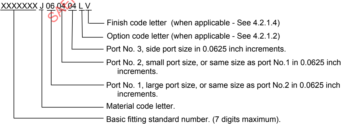
FIGURE 13 - PART NUMBER STRUCTURE FOR TEES WITH THE SAME STYLE PORTS OR WHEN THE DIFFERING PORT STYLE IS PORT NO. 3 STYLE
