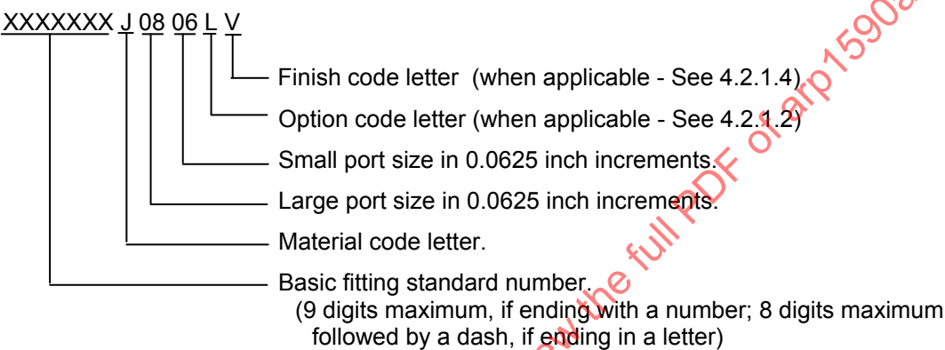
FIGURE 9 - PART NUMBER STRUCTURE FOR 2 PORT REDUCER/EXPANDER FITTINGS WITH BOTH PORTS THE SAME STYLE
