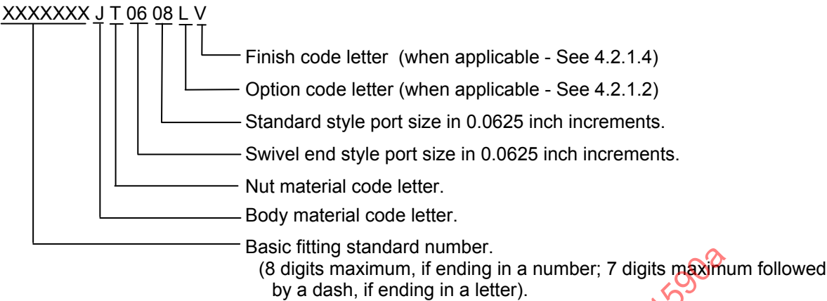
FIGURE 11 - PART NUMBER STRUCTURE FOR 2 PORT REDUCER/EXPANDER FITTING ASSEMBLIES
