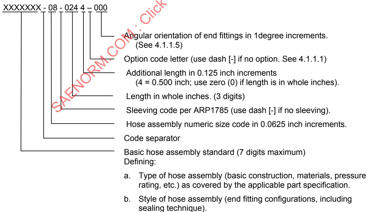
FIGURE 5 - 19 DIGIT PART NUMBER STRUCTURE FOR NON-REDUCING HOSE ASSEMBLIES
