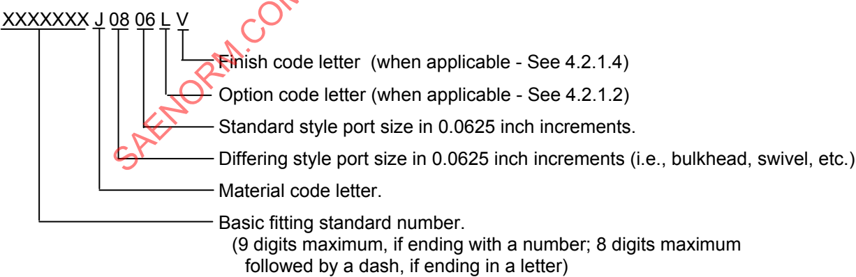
FIGURE 10 - PART NUMBER STRUCTURE FOR 2 PORT REDUCER/EXPANDER FITTINGS WITH DIFFERENT STYLE PORTS
