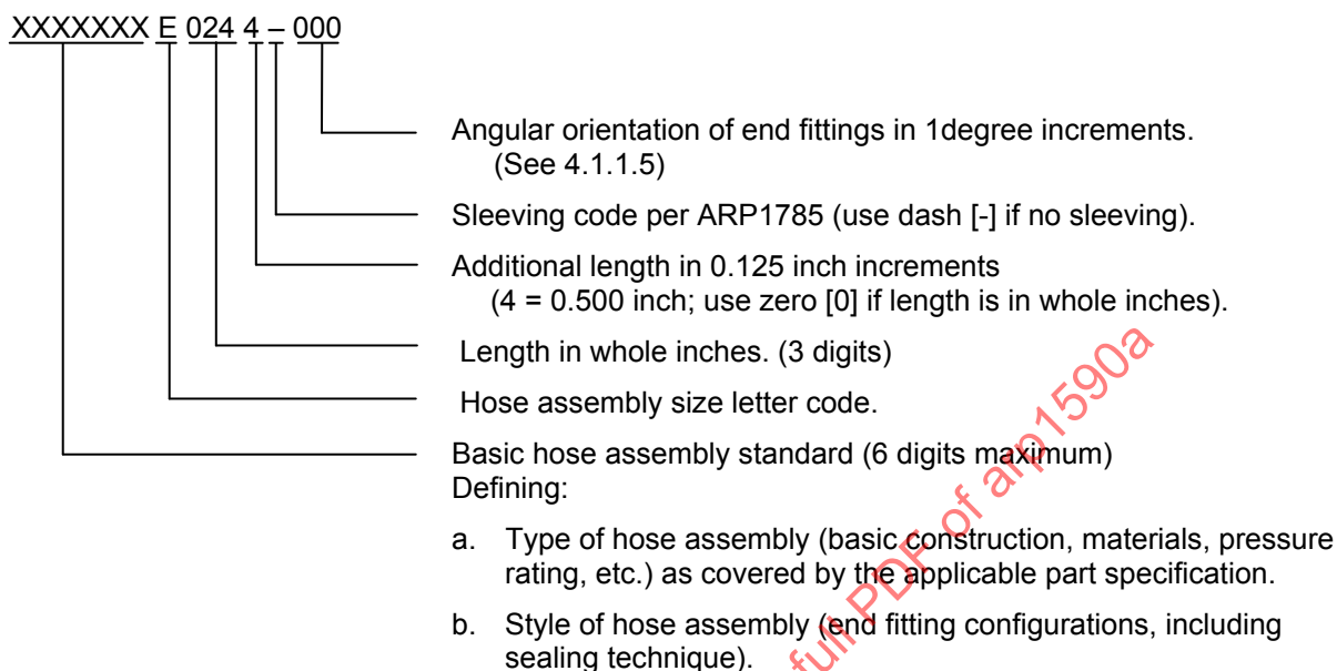
FIGURE 4 - 15 DIGIT PART NUMBER STRUCTURE FOR HOSE ASSEMBLIES WITH ELBOW AT BOTH ENDS
