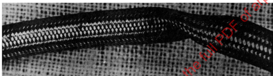
FIGURE 26 - Twist - Minor and Major Low and Medium Pressure PTFE Hose (MIL-H-25579/MIL-H-27267, AS620, AS1227, or AS1946)
