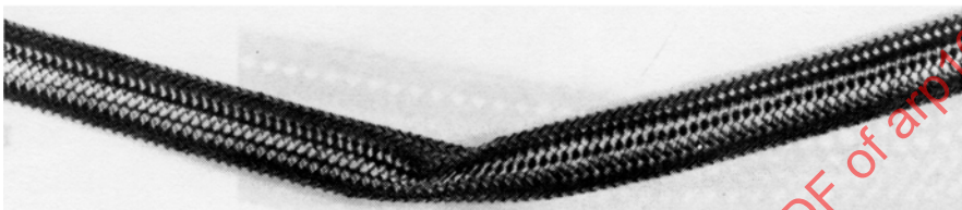
FIGURE 5 - Kinked Assemblies - Minor and Major Low and Medium Pressure PTFE Hose (MIL-H-25579/MIL-H-27267, AS620, AS1227, or AS1946)
