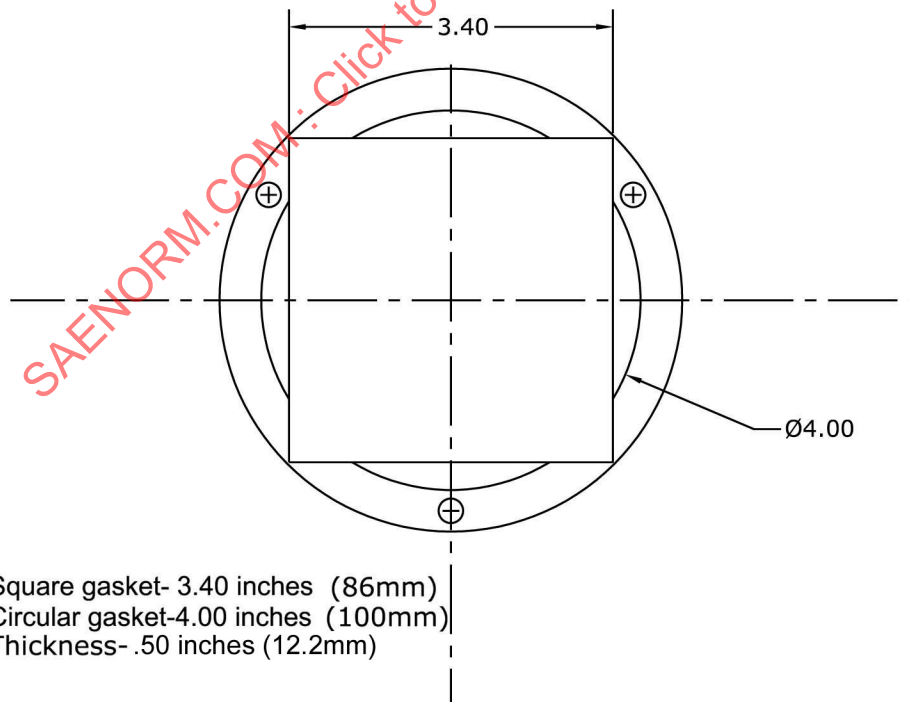
FIGURE B13 - MAXIMUM GASKET DIMENSIONS
