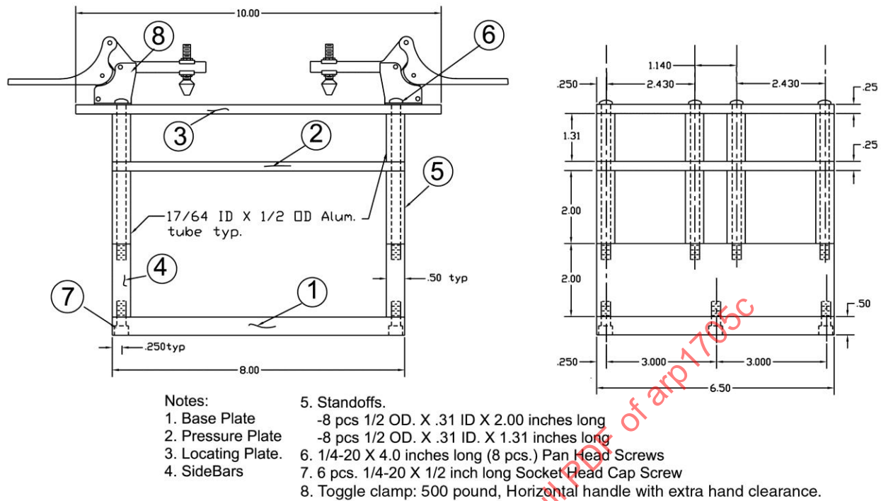
Figure B8 - Frame assembly
