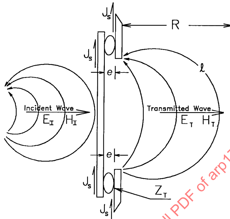
Figure 1 - Penetration of EM wave through EMI gasketed maintenance cover
