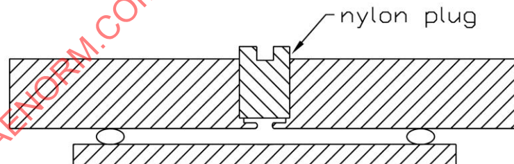
Figure B1 - 1705A test fixture (gasket assembly under test)
