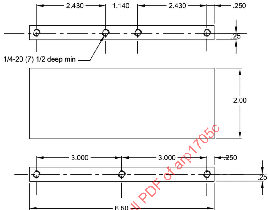
Figure B12 - Side bars
