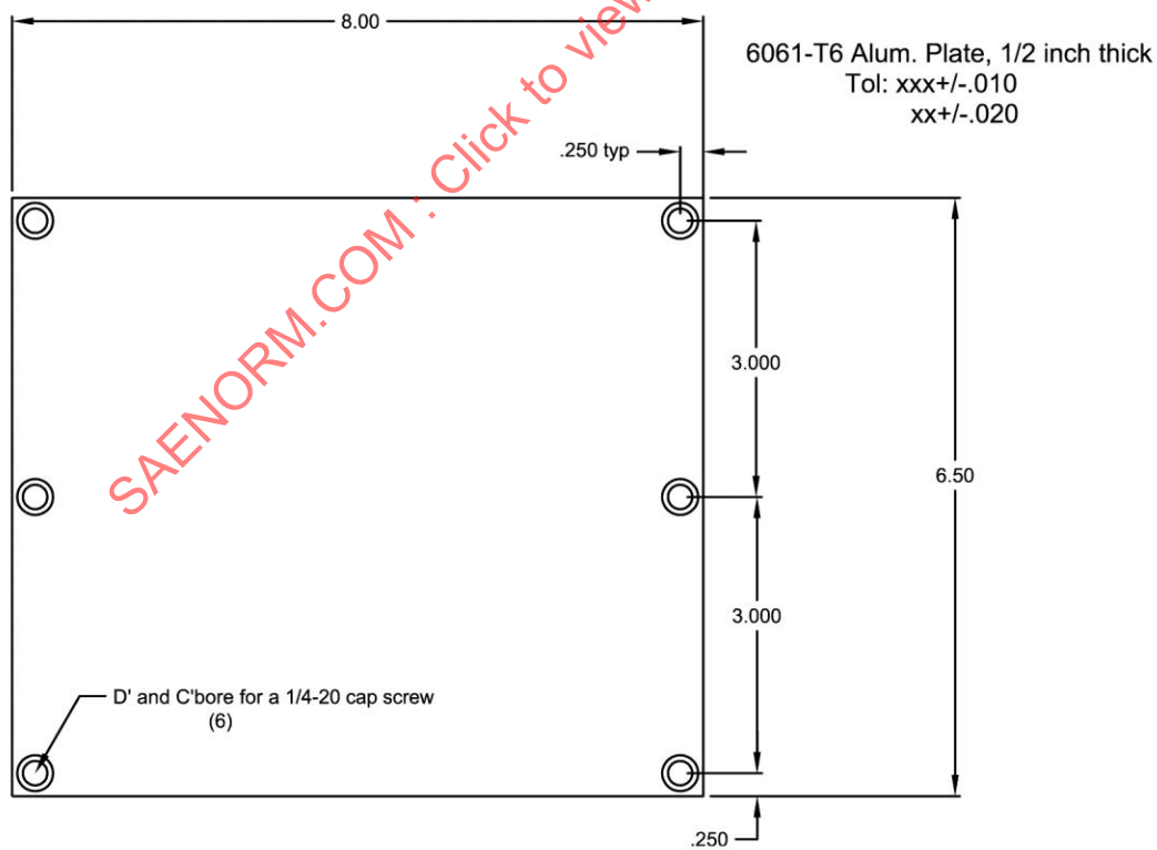
Figure B9 - Fixture base plate
