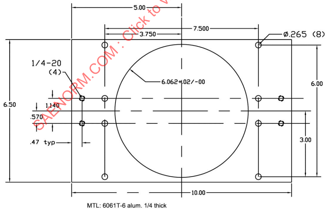
Figure B11 - Locating plate
