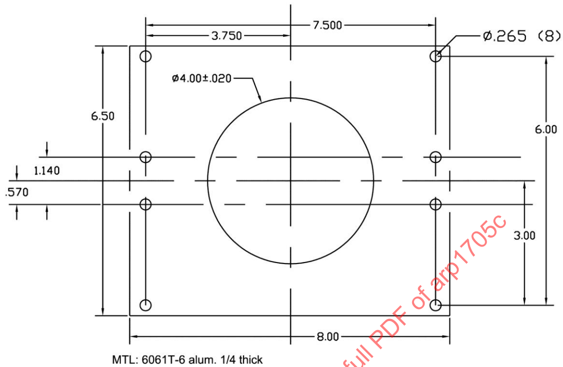
Figure B10 - Pressure plate
