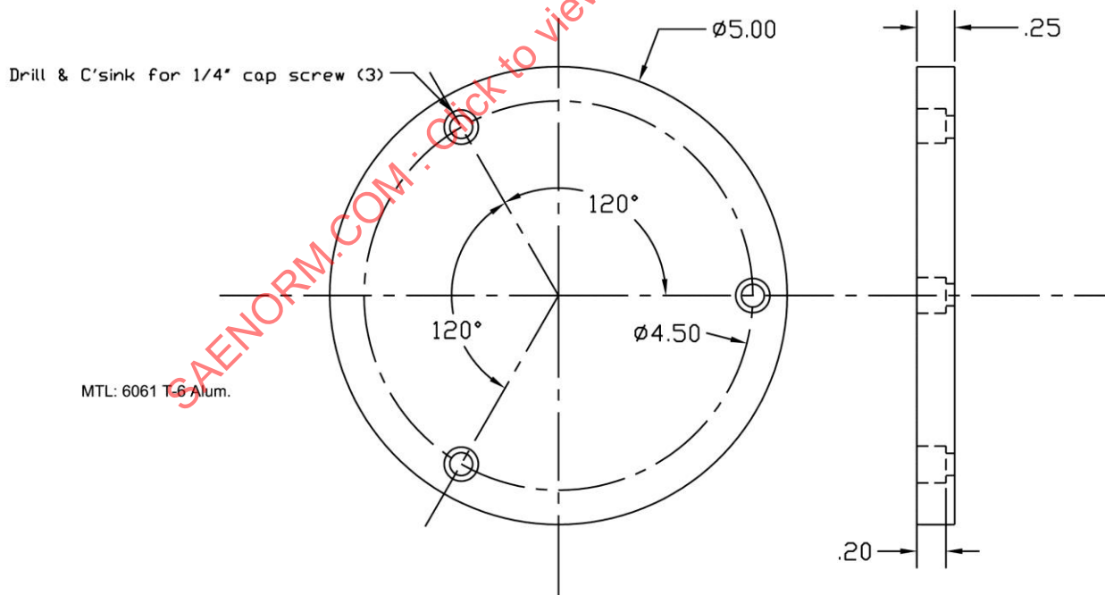
Figure B3 - Contact plate
