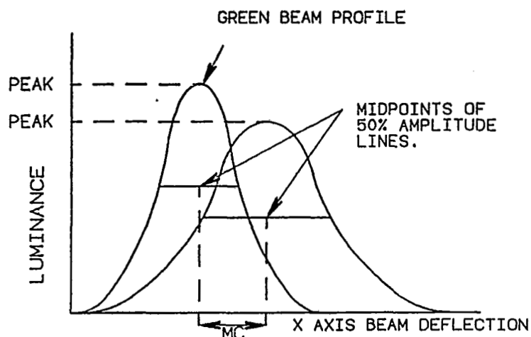
FIGURE 5A - Illustration of Misconvergence (MC) of Two Primary Beams (Green and Red or Blue)
