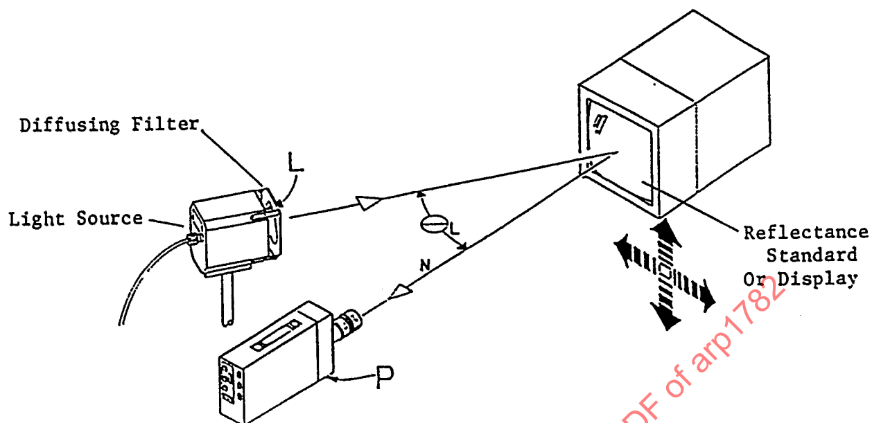
FIGURE 20 - Diffuse Configuration for Measuring Reflectance at Display From an Off-Axis Source
