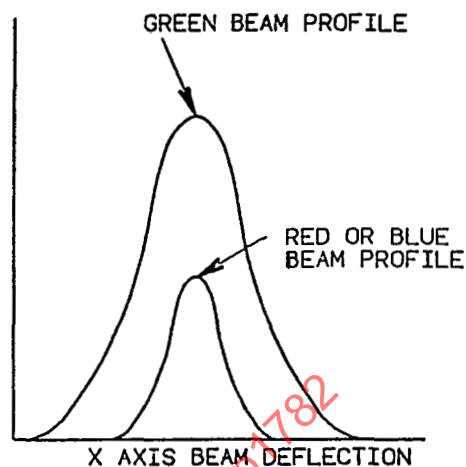
FIGURE 5B - Apparent Misconvergence of Two Primary Beams
