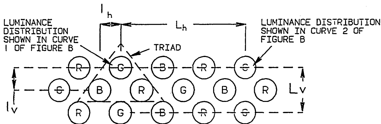
FIGURE 6A - Phosphor Dots on Shadowmask CRT Display
