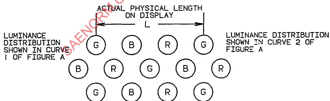
FIGURE 4B - Phosphor Dots on Shadowmask CRT Display
