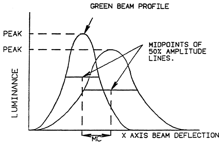
FIGURE 5A - Illustration of Misconvergence (MC) of Two Primary Beams (Green and Red or Blue) (Scale Factor Per Figs. 4A and 4B Taken Into Account)
