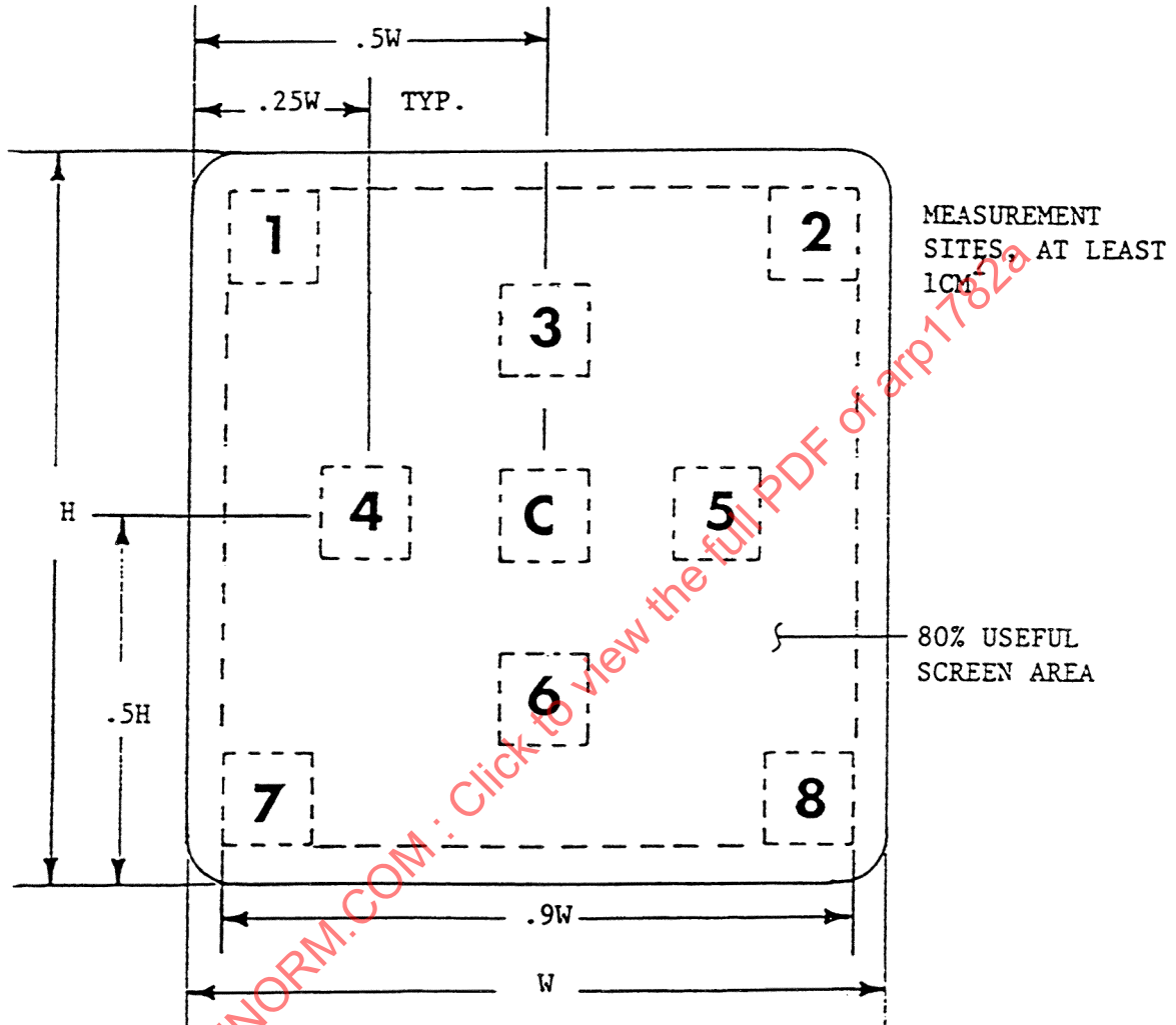
FIGURE 18 - Site Measurement Pattern for Luminance and Color Uniformity
