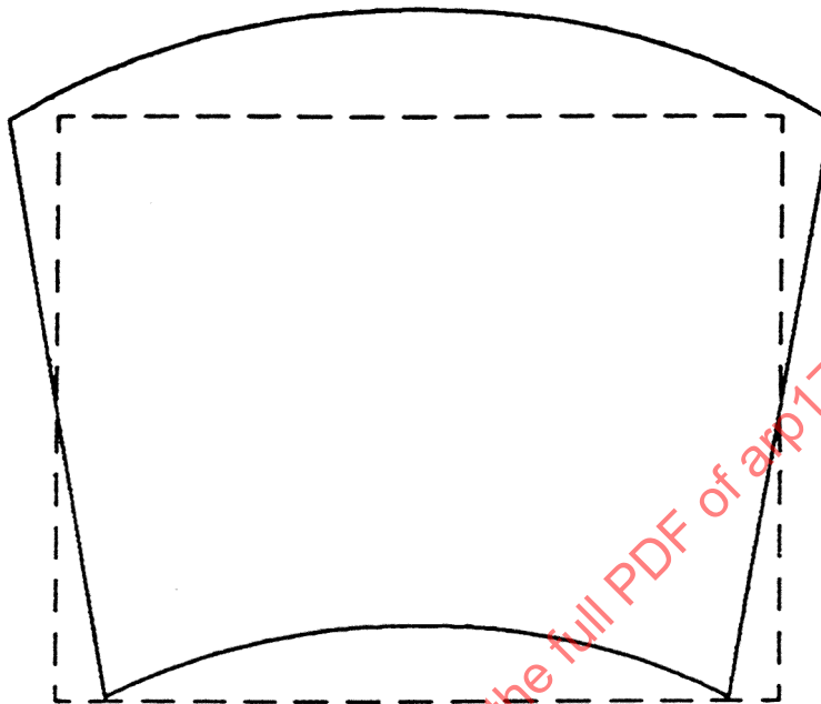
FIGURE 12 - Keystone/Pincushion/Barrel Distortion
