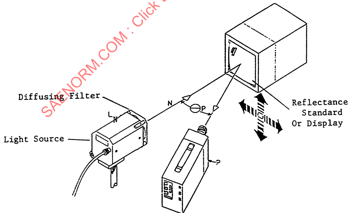
FIGURE 21 - Diffuse Configuration for Measuring Reflectance at Display Surface From Light Source Normal to Display
