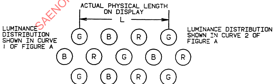
FIGURE 4B - Phosphor Dots on Shadowmask CRT Display
