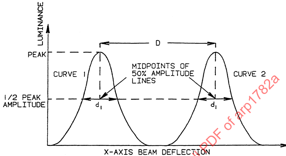
FIGURE 4A - Determine Scale Factor and Line Width
