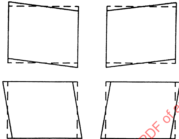
FIGURE 10 - Orthogonality Distortion
