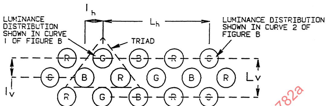
FIGURE 6A - Phosphor Dots on Shadowmask CRT Display
