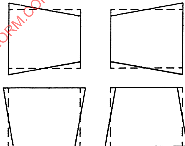
FIGURE 9 - Keystone Distortion
