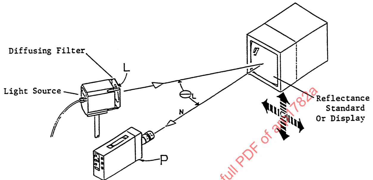
FIGURE 20 - Diffuse Configuration for Measuring Reflectance at Display From an Off-Axis Source
