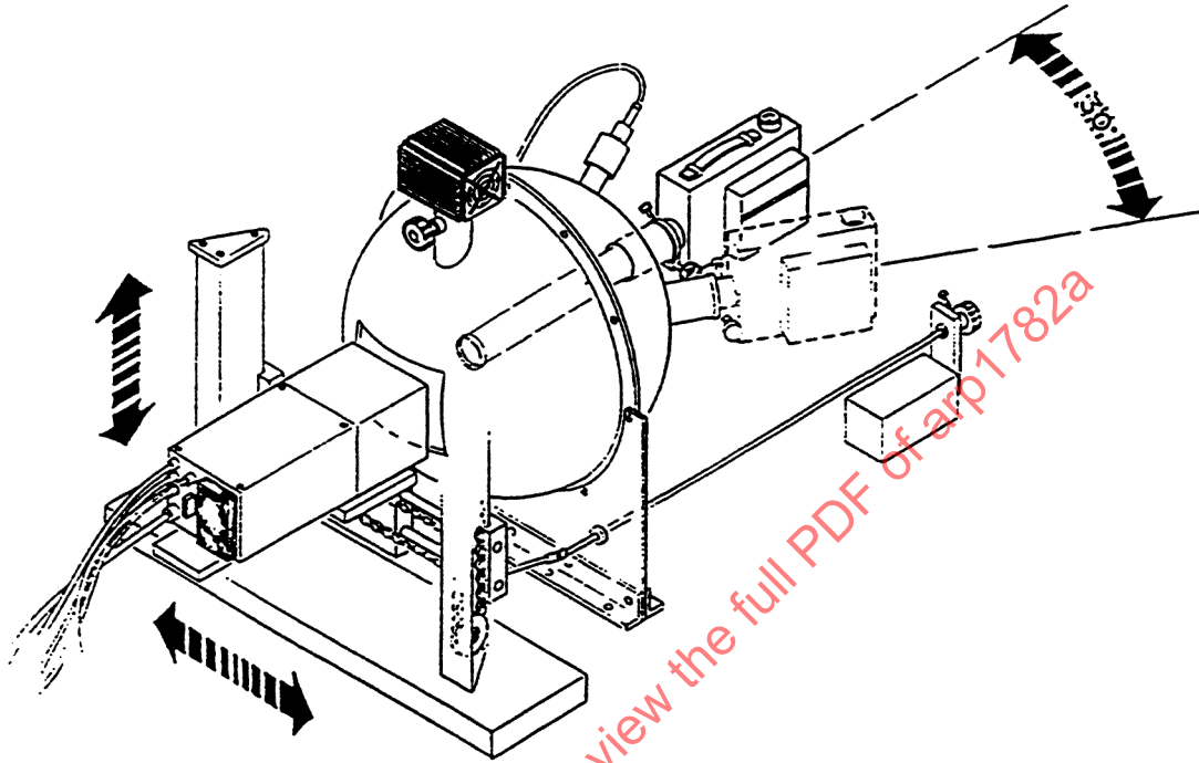
FIGURE 23 - Typical Integrating Sphere High Intensity Diffuse Light Source for Display Contrast Measurements
