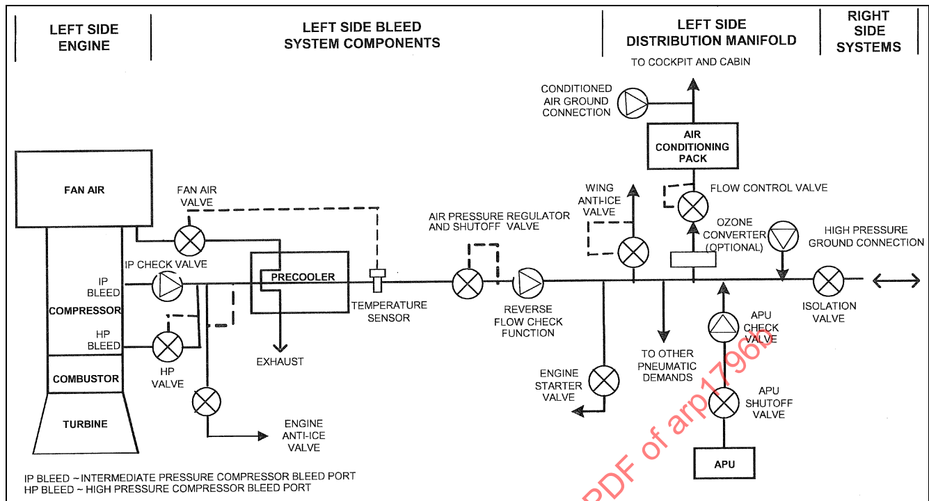
Figure 1 - Typical aircraft bleed air system
