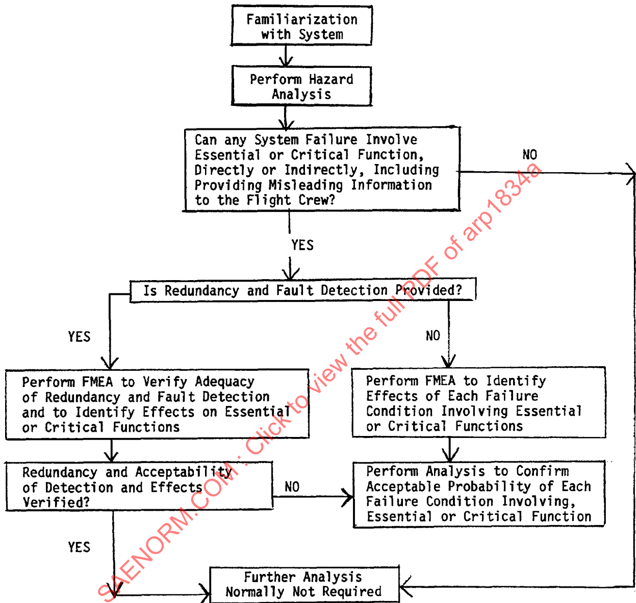
FIGURE 3 - An Example of a F/FA Decision Tree
