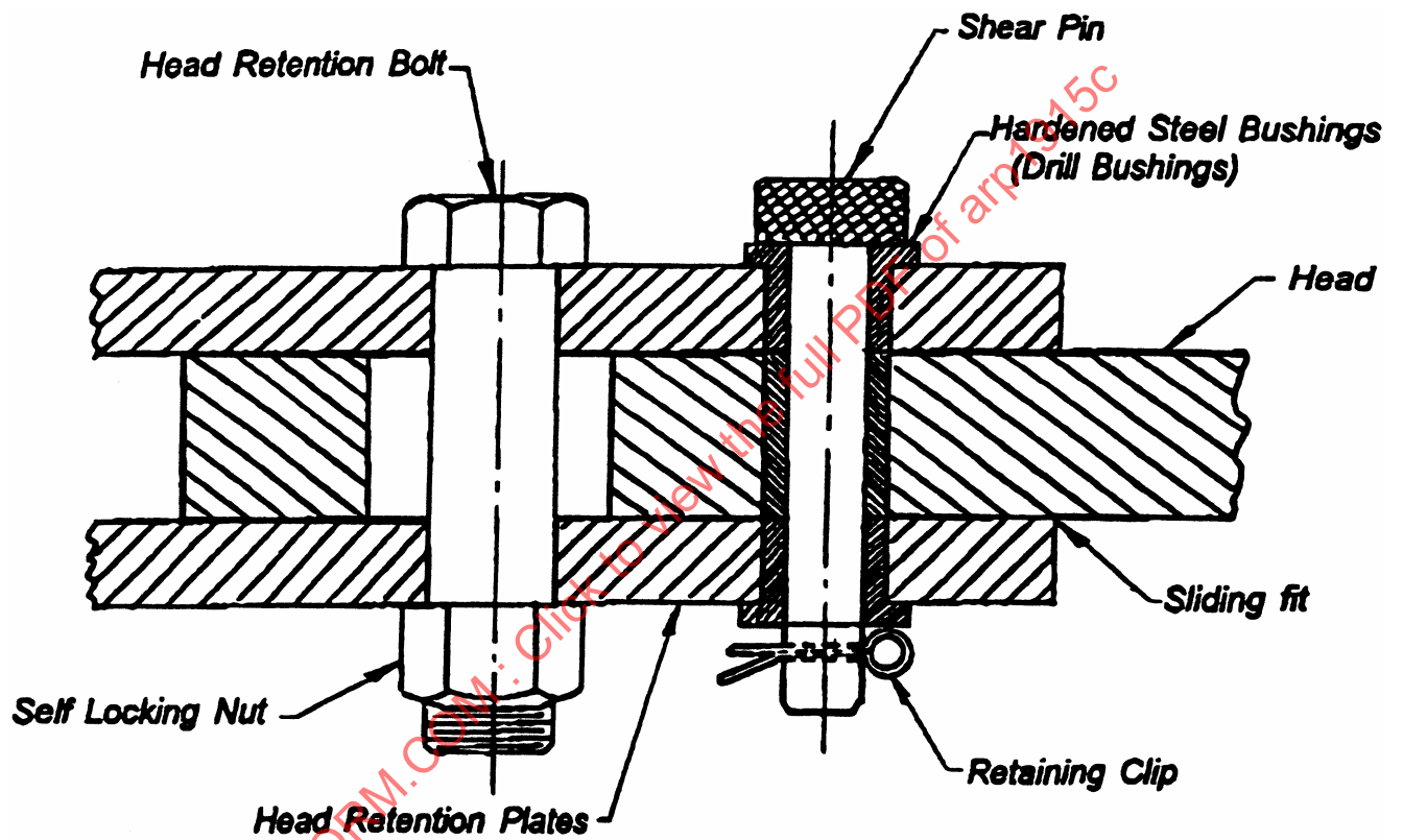
FIGURE 3 - Typical Shear Pin, Bushings, and Head Retention Bolt Configuration
