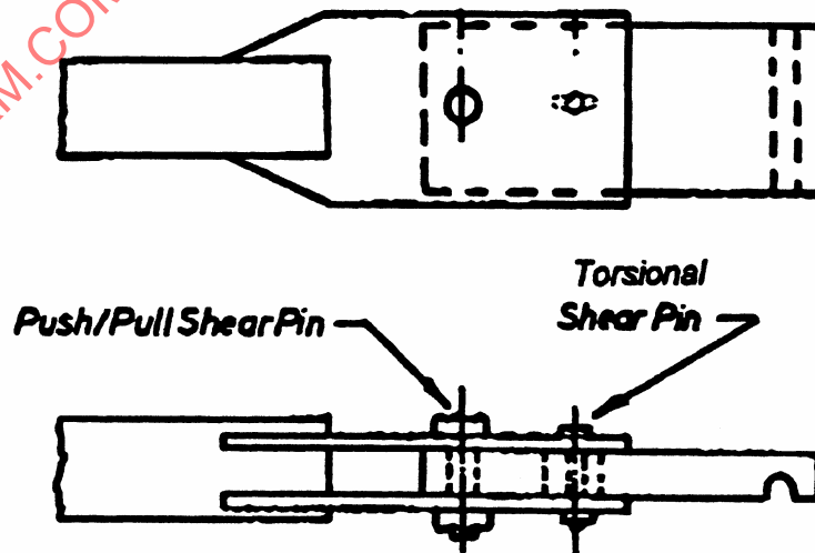
FIGURE 5 - Single Function Shear Pins
