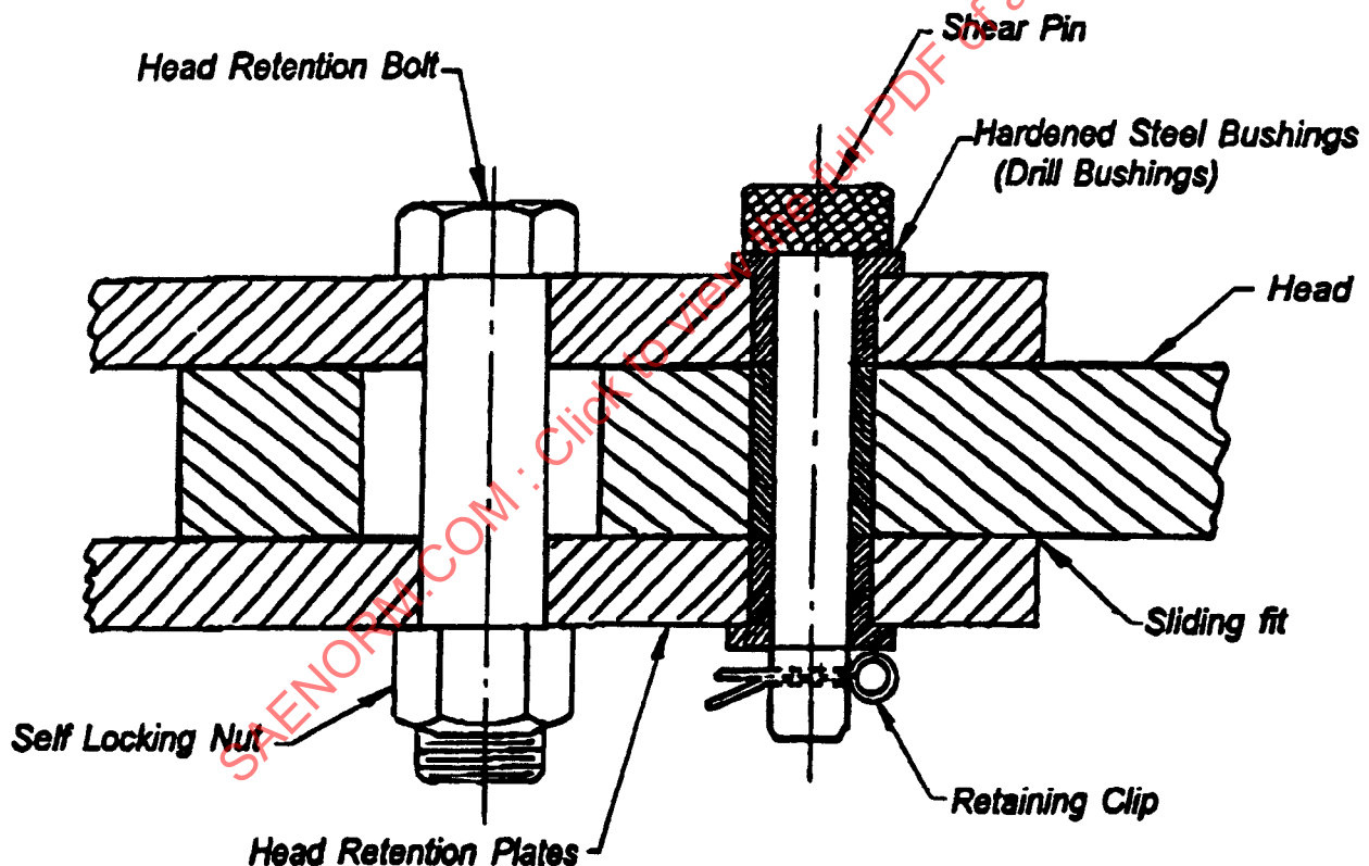
FIGURE 3 - TYPICAL SHEAR PIN, BUSHINGS, AND HEAD RETENTION BOLT CONFIGURATION (ILLUSTRATION ONLY)
