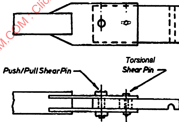
FIGURE 5 - SINGLE FUNCTION SHEAR PINS (ILLUSTRATION ONLY)
