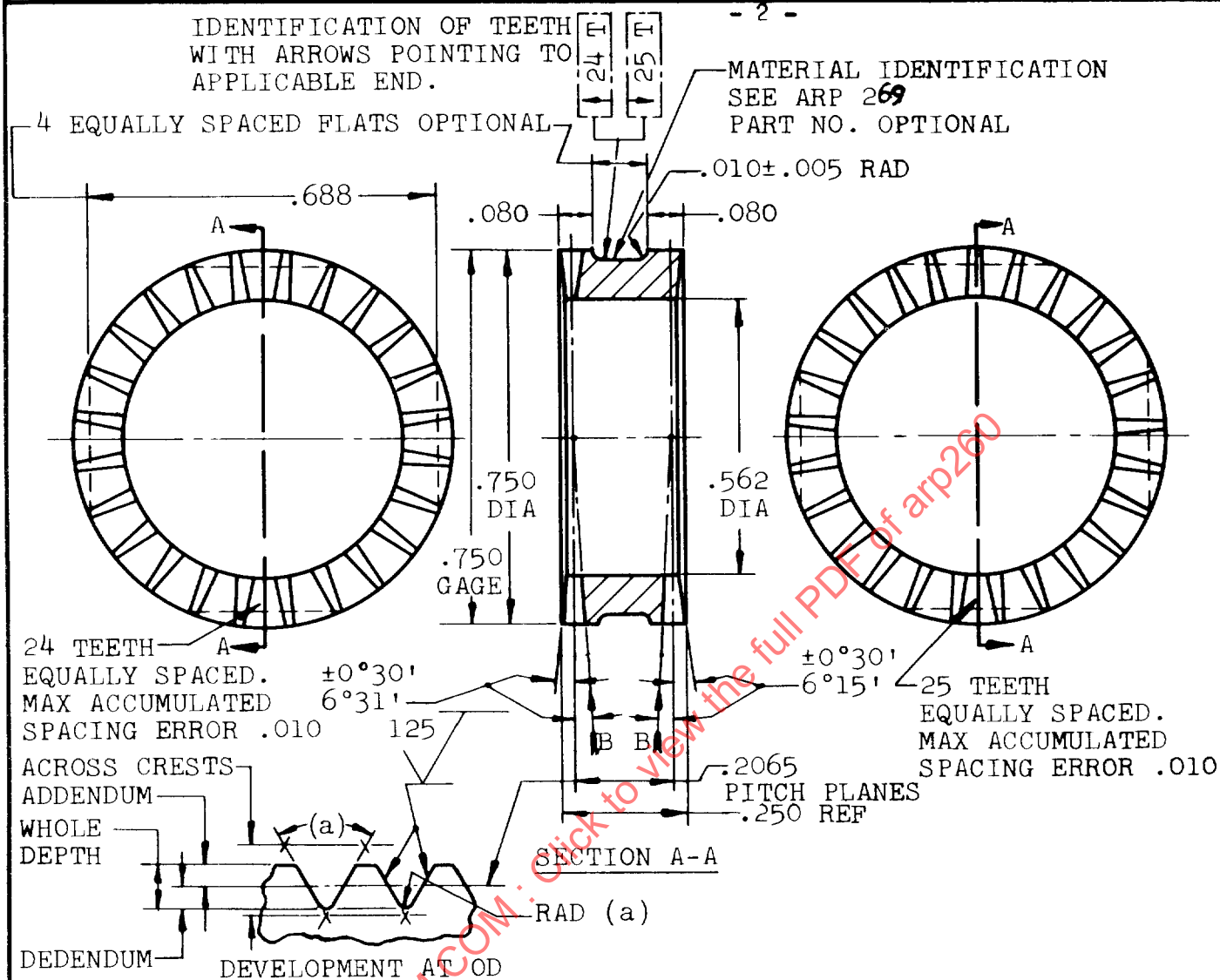
SERRATED FACE COUPLING DATA AT .750 DIA
