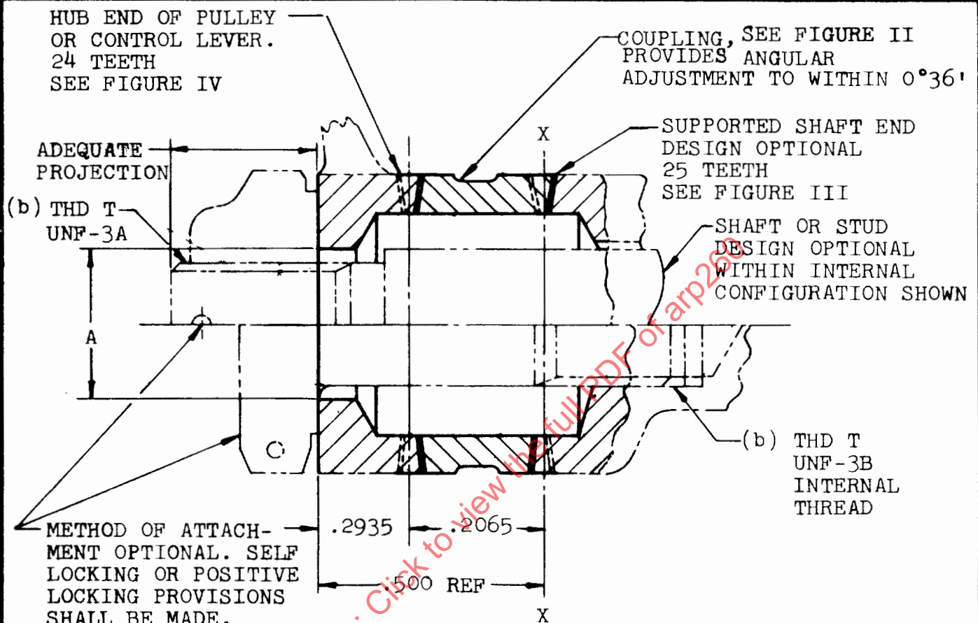
FIGURE I INSTALLATION
