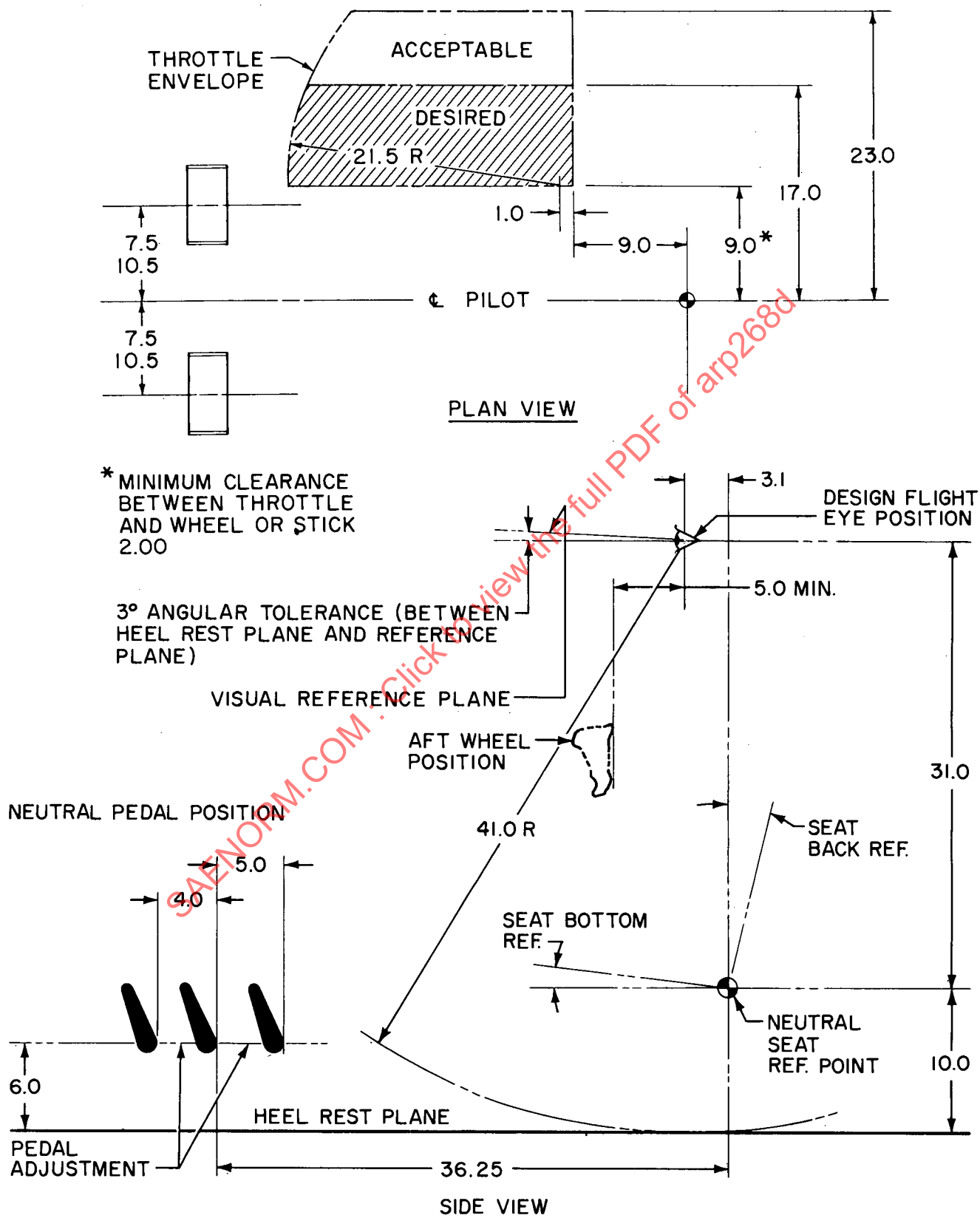
FIGURE 2 - PILOT'S NORMAL POSITION
