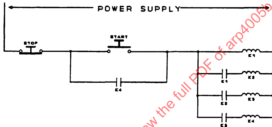
FIGURE 4 - CONCURRENT RELAY OPERATION, CASCADE METHOD
