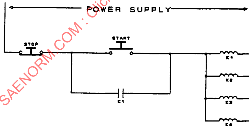
FIGURE 5 - CONCURRENT RELAY OPERATION, PARALLEL METHOD
