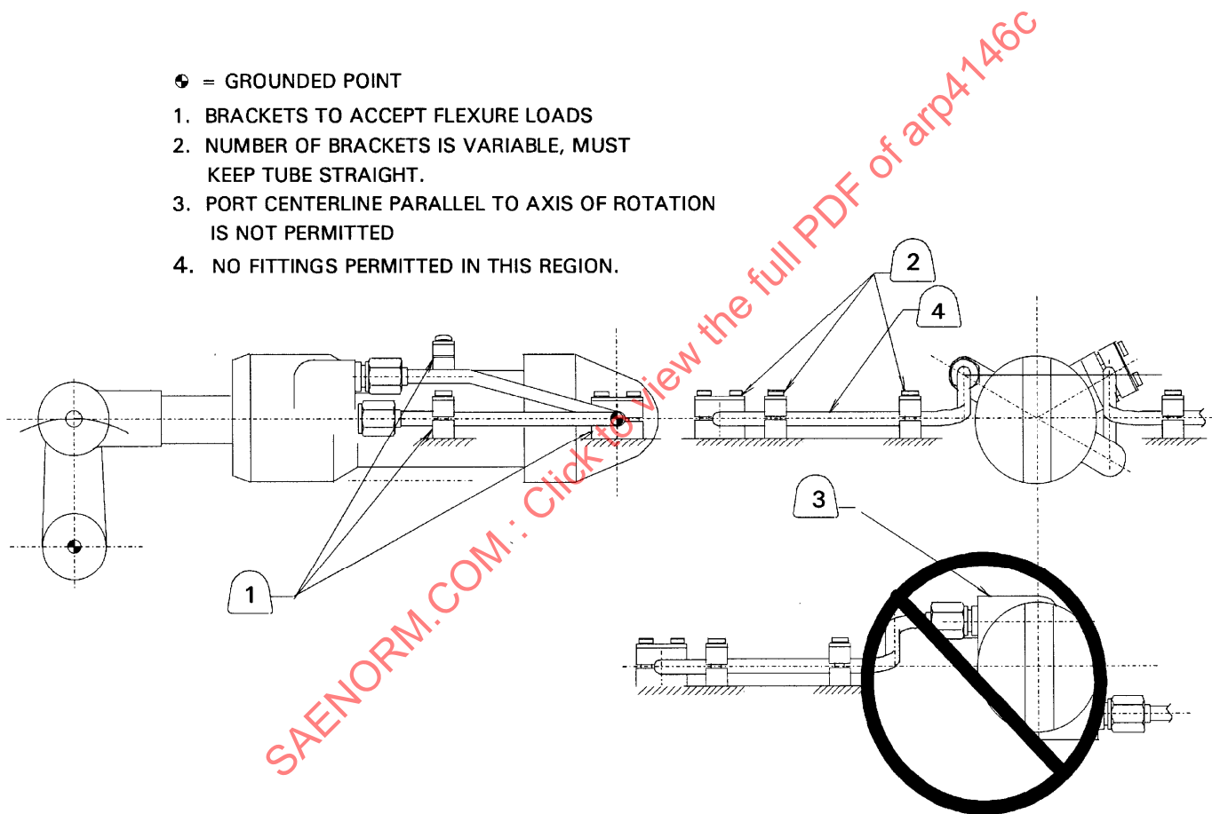
FIGURE 2 - STYLE B - TORSION TUBE CONFIGURATION
