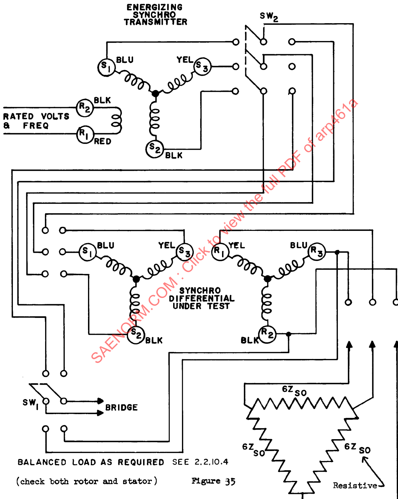
Temperature Rise Test for Differential Transmitters and Differential Receivers
