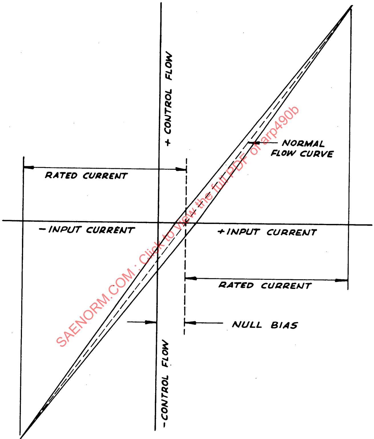
Figure 2. Normal Flow Curve
