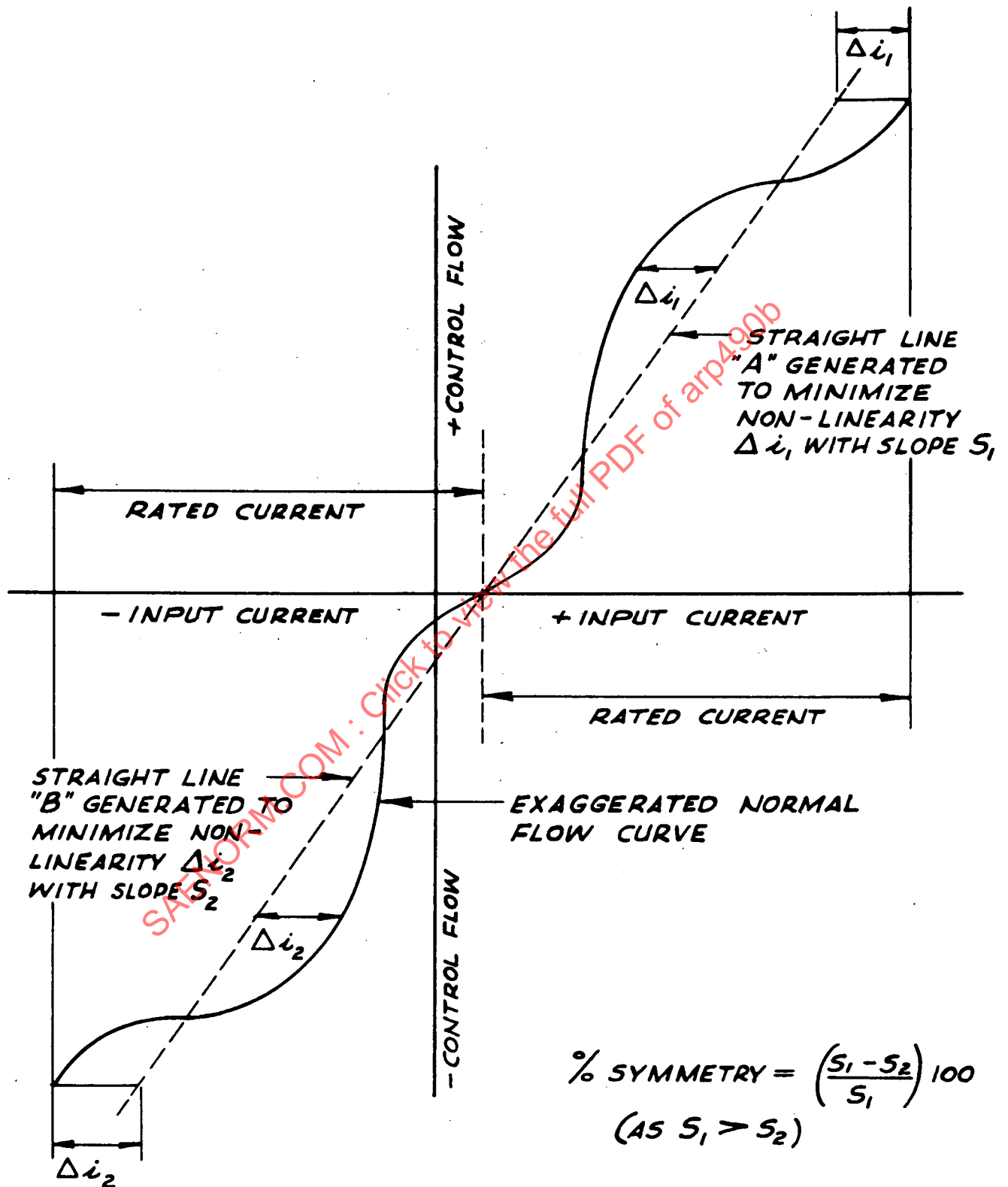
Figure 4. Linearity/Symmetry
