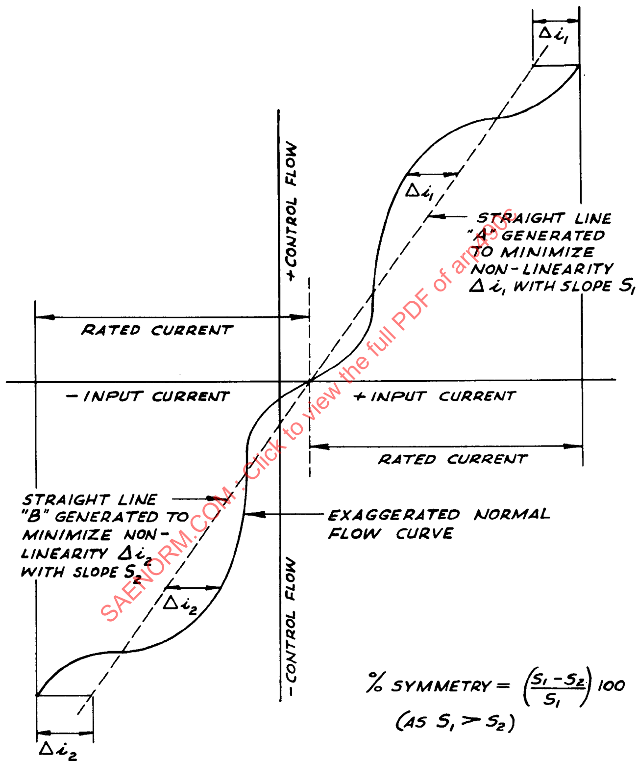
Figure 4. Linearity/Symmetry
