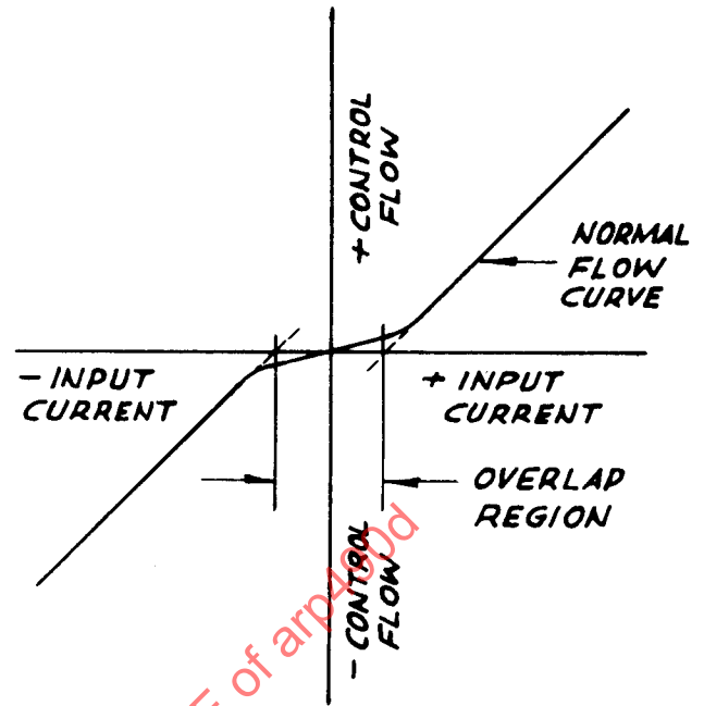
Figure 6B. Overlap
