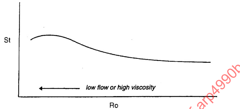
Figure 3 - Strouhal-Roshko relationship
