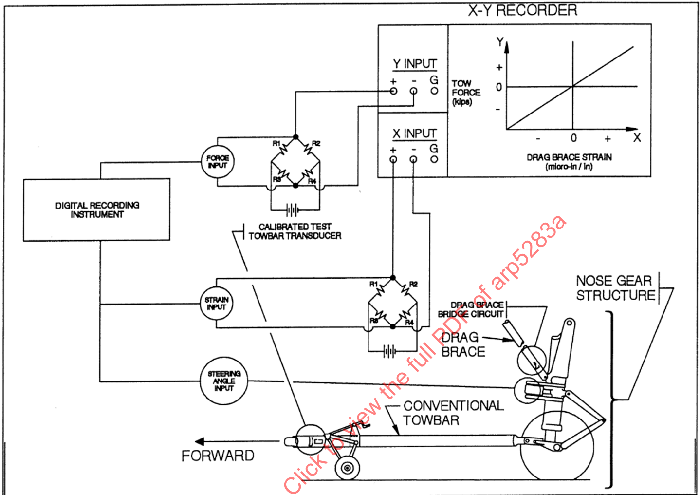
FIGURE 1 - TOW LOAD
