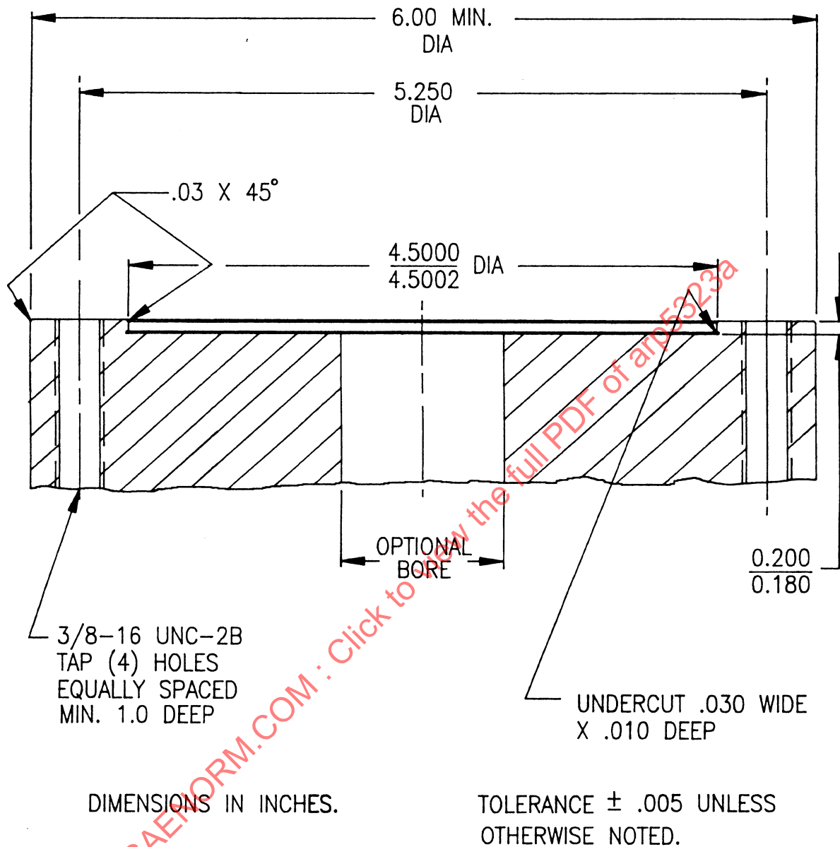
Figure A3 - Spindle flange, machine class 50, 100, 250, 500
