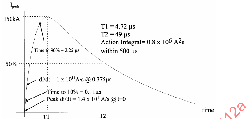
FIGURE 14A - Current Component A_h for Analysis Purposes
