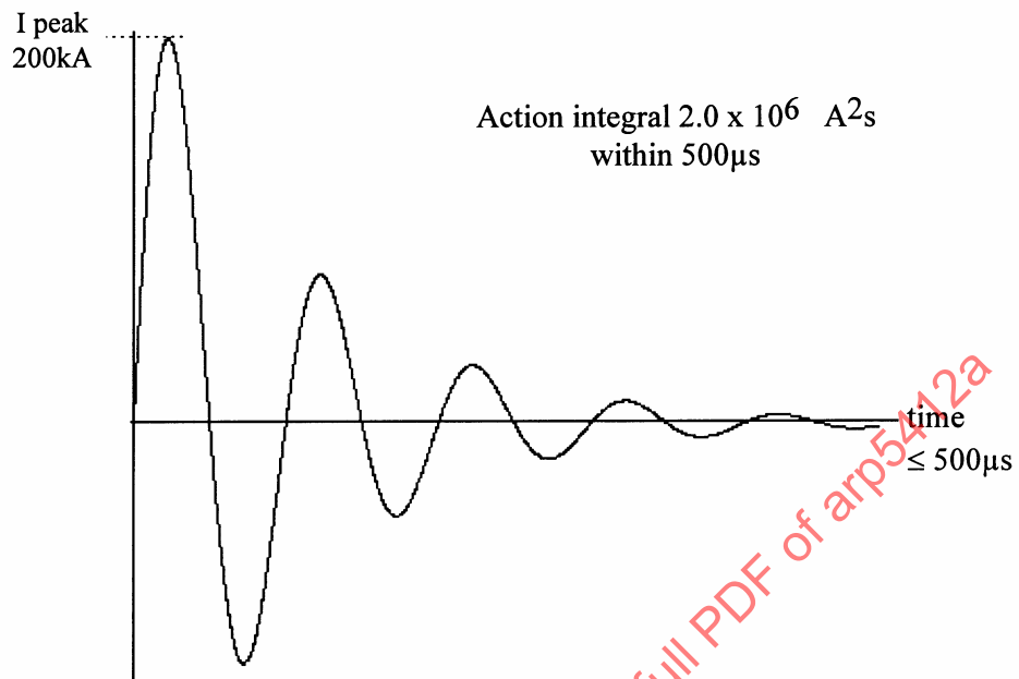
FIGURE 13A - Damped Sinusoidal Current
