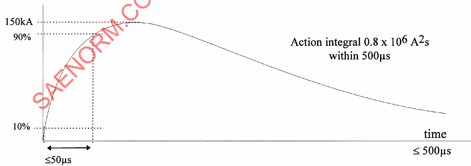
FIGURE 14C - Example for Current Component A_h for Direct Effects, Unipolar Current
