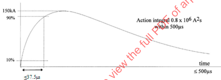
FIGURE 15B - EXAMPLE FOR CURRENT COMPONENT A_H FOR DIRECT EFFECTS, UNIPOLAR CURRENT
