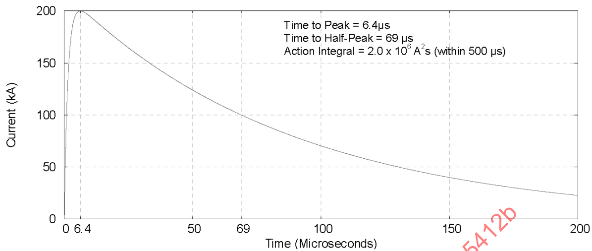
(A) TIME DOMAIN WAVEFORM TO 200 MICROSECONDS
