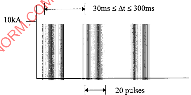
FIGURE 11 - MULTIPLE BURST WAVEFORM SET
