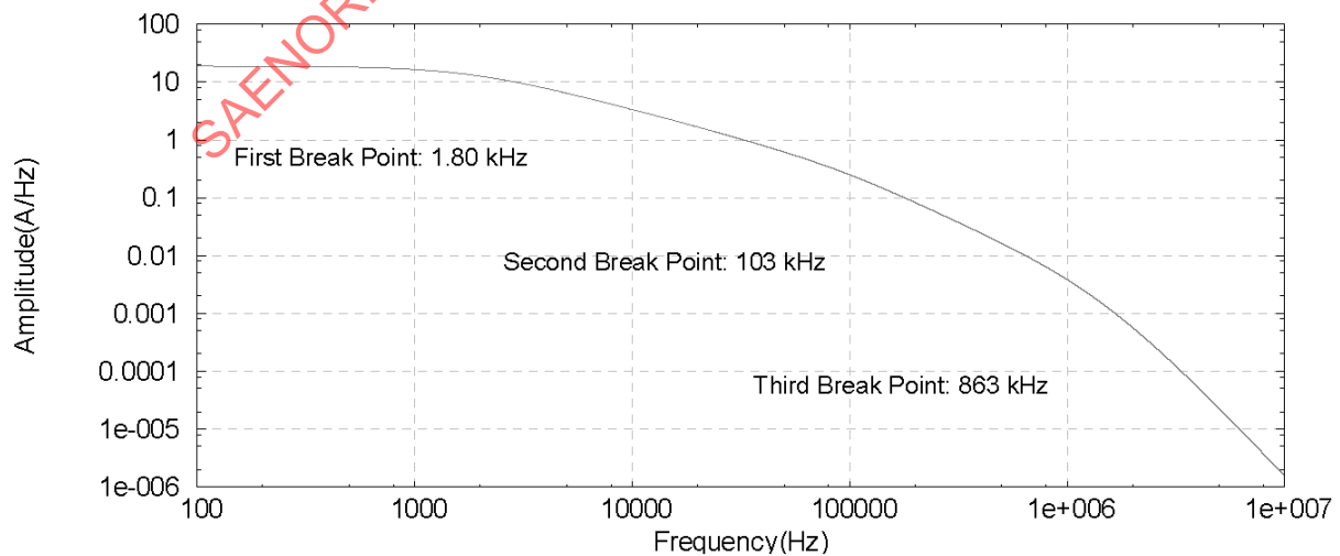
(C) FREQUENCY CONTENT (AMPLITUDE SPECTRUM)
