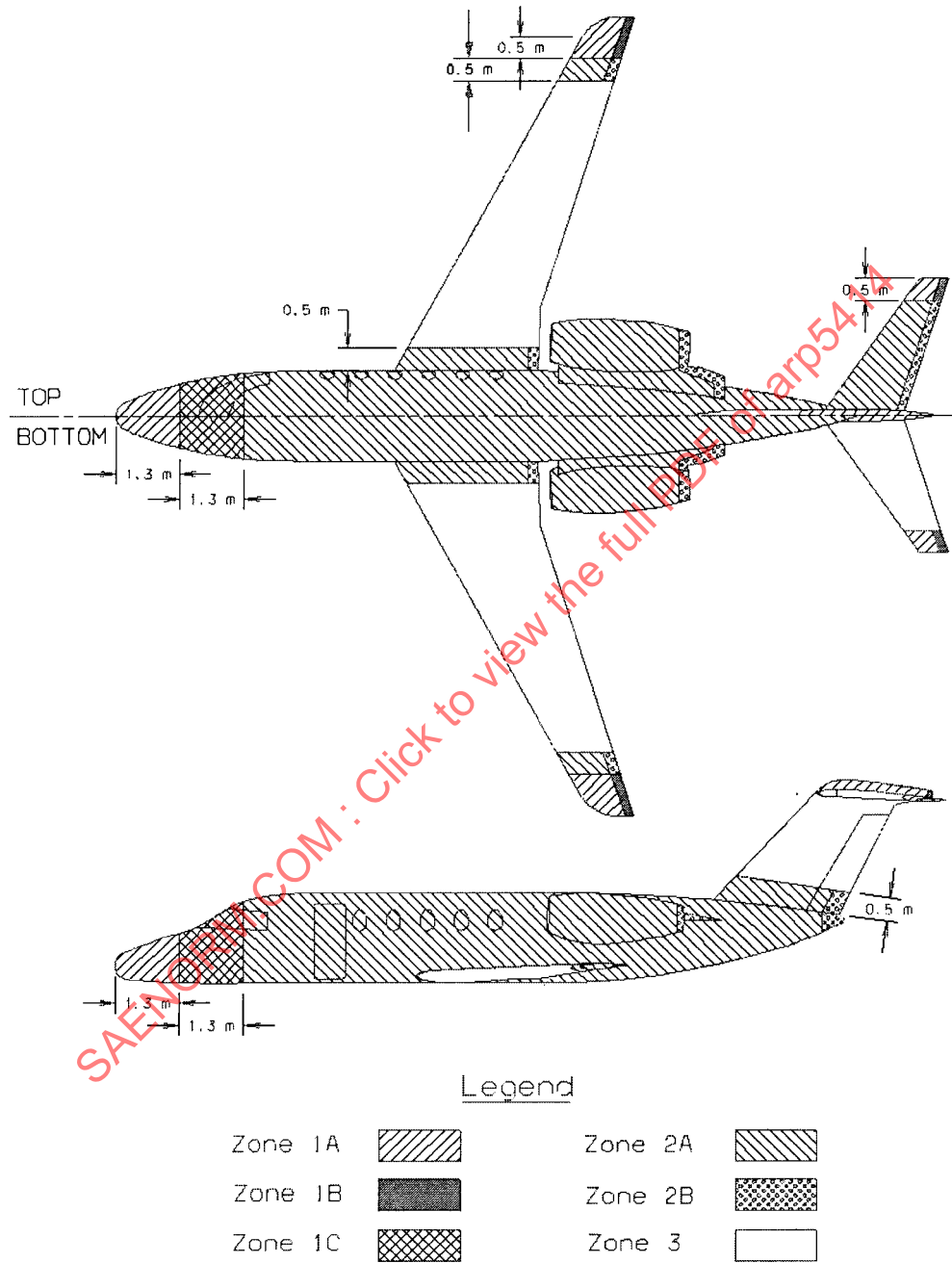
FIGURE 10 - Example of Lightning Strike Zone Details for Swept Wing Business Jet
