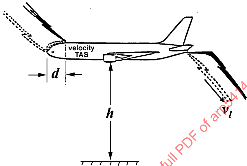
FIGURE 5 - Leader Sweep, Aircraft Altitude and Aircraft Leader Velocities
