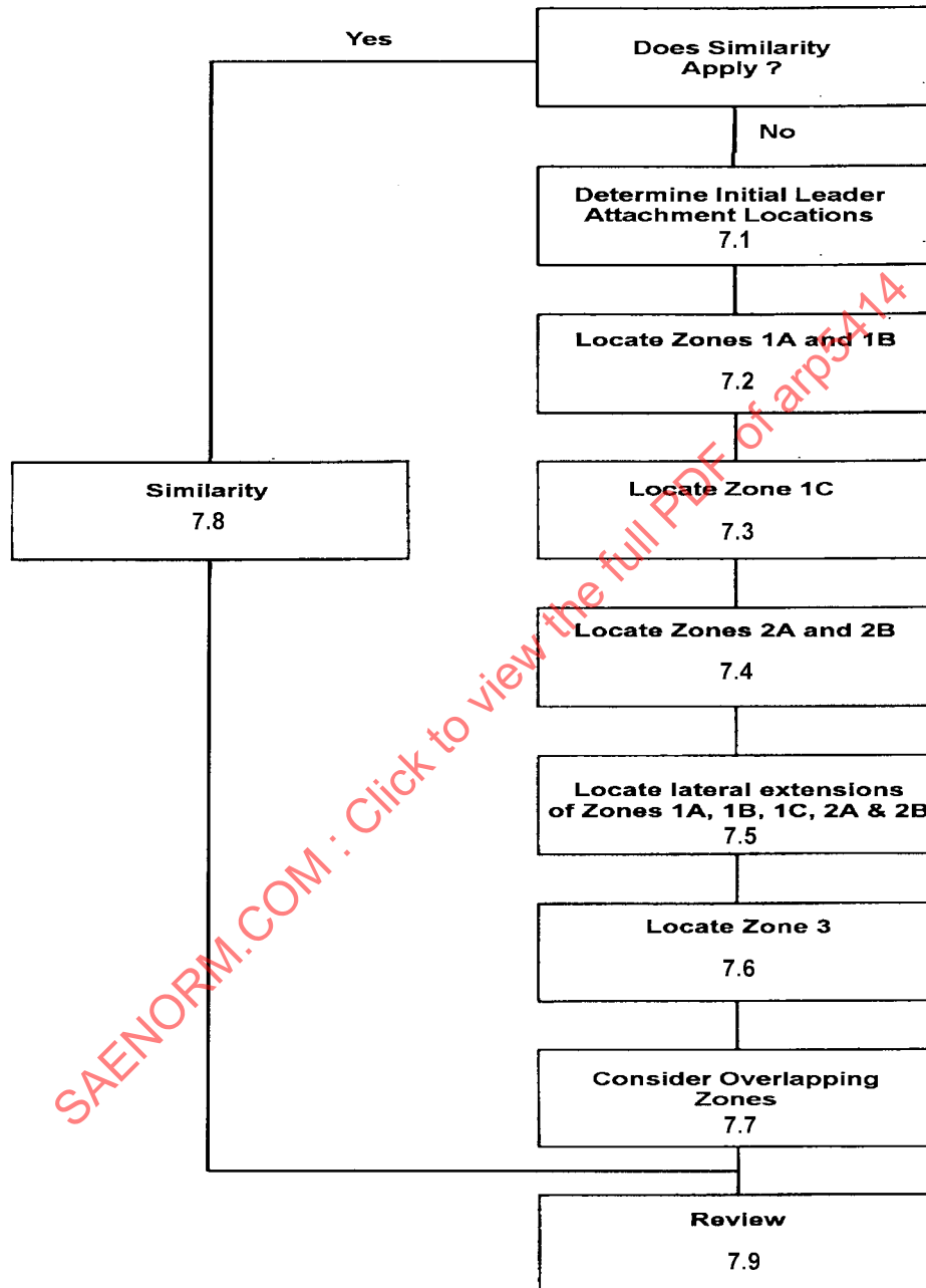
FIGURE 4 - Zone Location Process
