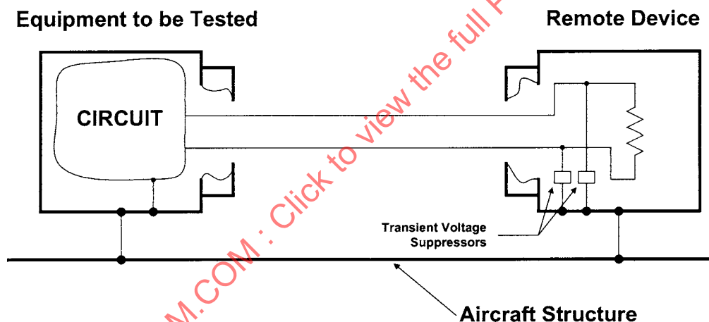
FIGURE 7 - Equipment Pins With Remote Transient Voltage Suppressors
