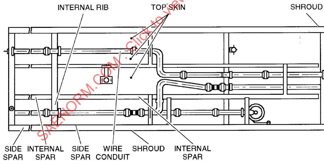
FIGURE B21 - Locations Where Currents Were Measured
