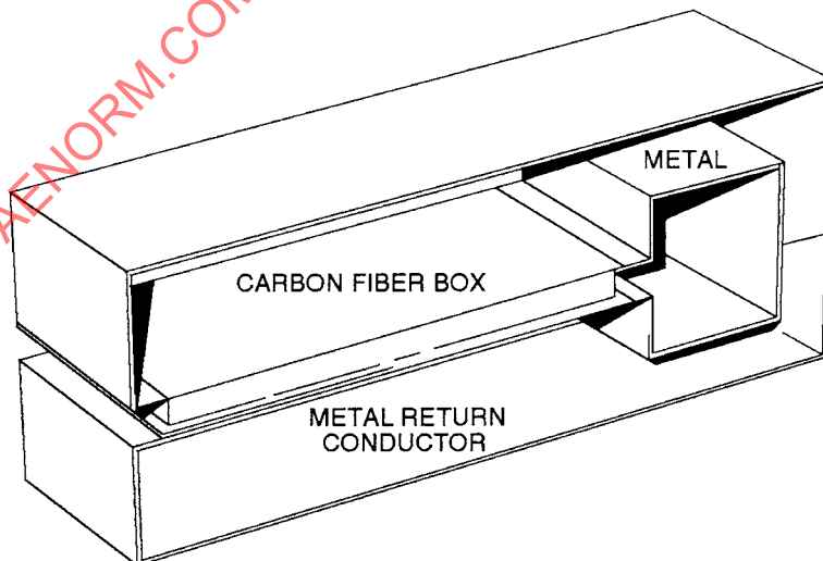
FIGURE B19 - Setup for Tests on Wing Box
