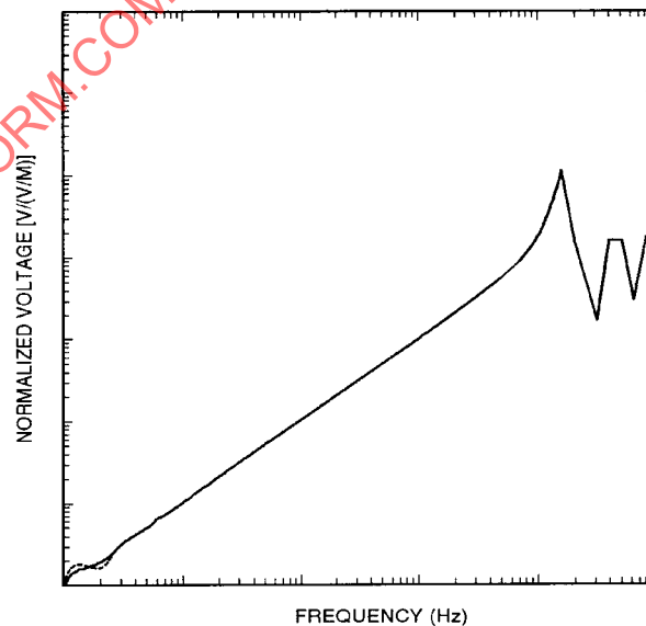
FIGURE B11 - Transfer Function - Open Circuit Configuration of a 1-Meter Long Wire Above a Ground Plane
