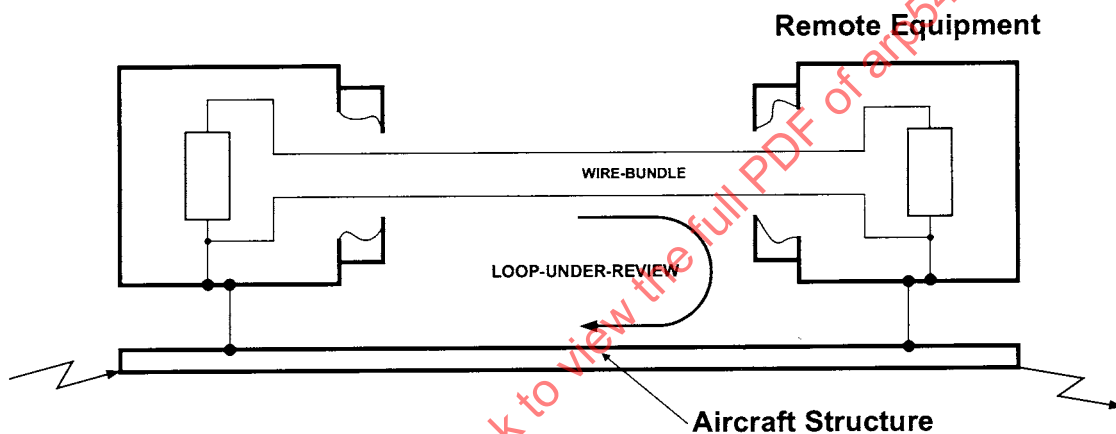
FIGURE 3 - Simple System Exposed to Lightning Induced Effects
