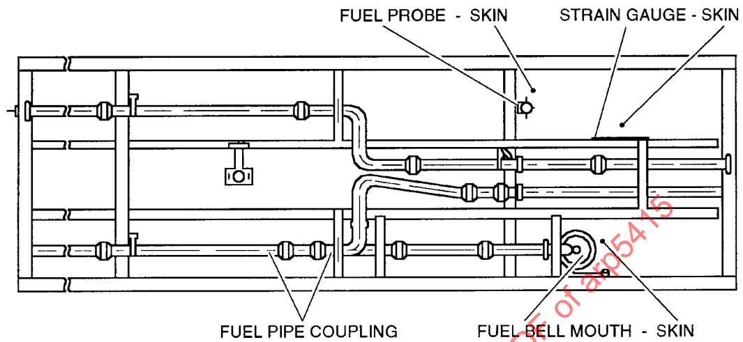
FIGURE B20 - Locations Where Voltages Were Measured
