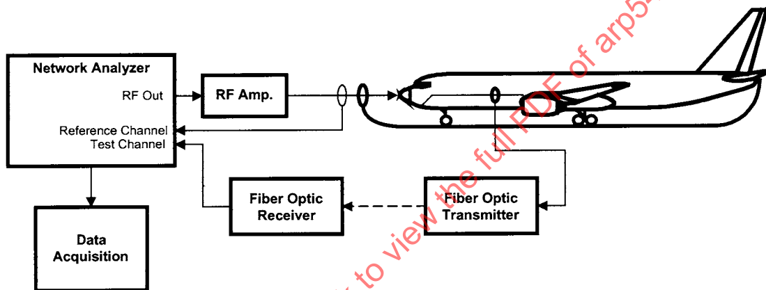
FIGURE 10 - Swept Frequency Test Setup
