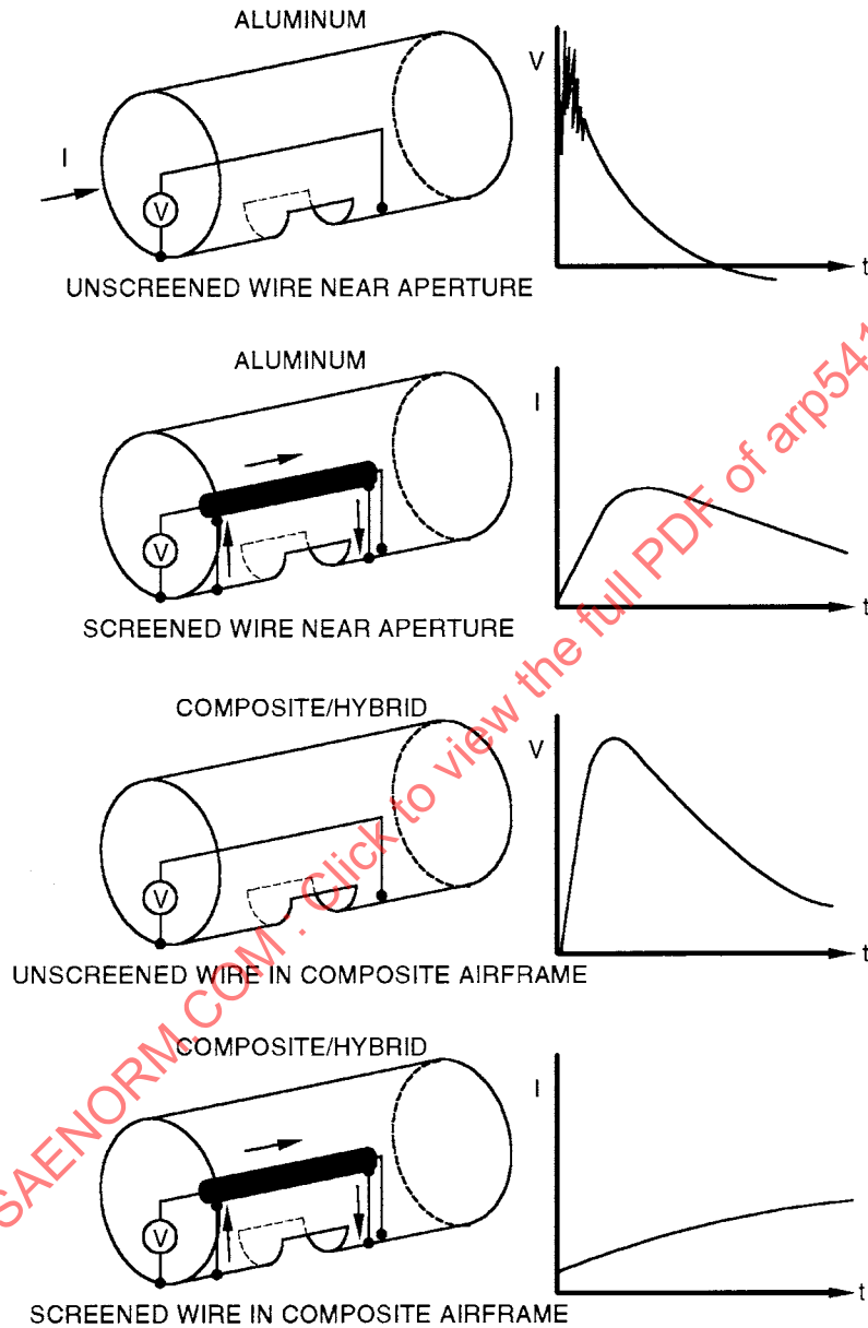
FIGURE B3 - Field Topology Effects on Coupling Mechanisms
