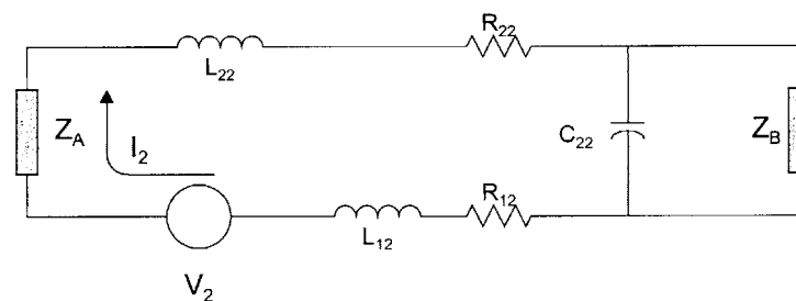
FIGURE B4 - Wire and Circuit Coupling Mechanisms
