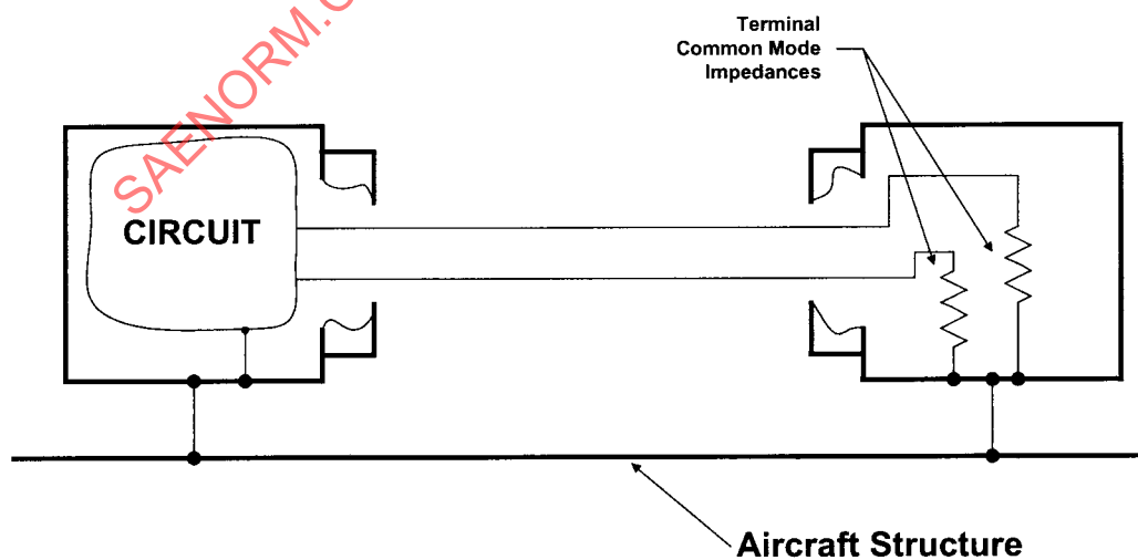
FIGURE 6 - Equipment Pins With Remote Circuits Referenced to Case/Aircraft Structure
