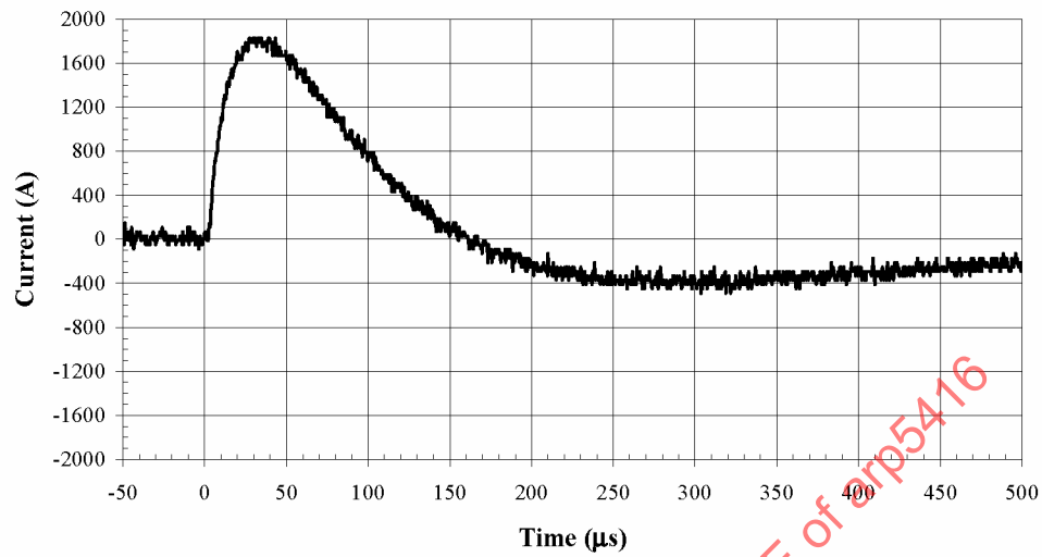
FIGURE 25 - Typical Wire Bundle Short Circuit Current Due to Current Component A
