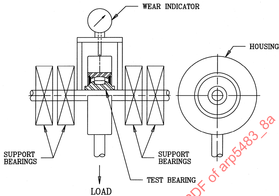
FIGURE 1 - TEST FIXTURE
