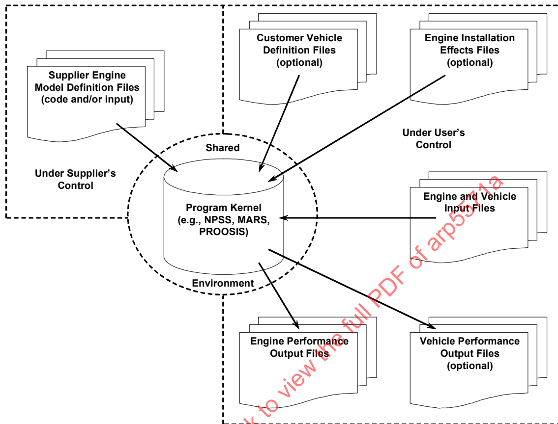
FIGURE 1 - SHARED/RESTRICTED-ENVIRONMENT ARCHITECTURE
