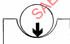
UNACCEPTABLE : Load bears onto a single point + low shoring stiffness
