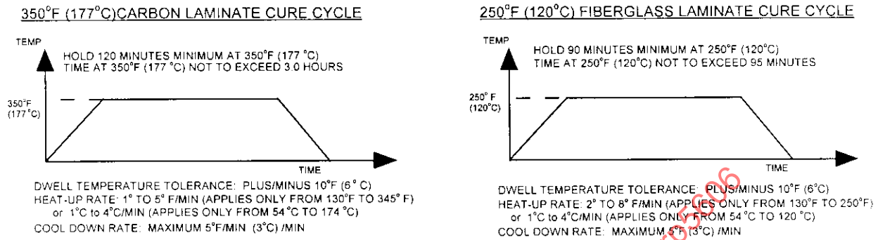
FIGURE 2 - Laminate Cure Temperature Profile
