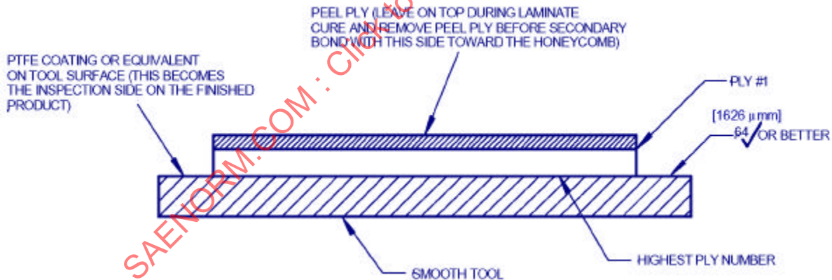
FIGURE 1 - Laminate Lay-Up on Smooth Tool
