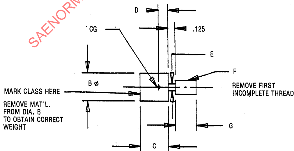
FIGURE A2 - Test Masses for 52 lb and Larger Proving Rotors
