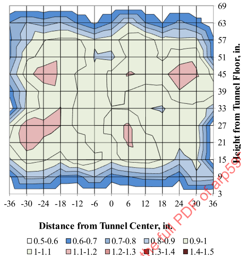
Figure 12 - Example of icing cloud uniformity and size data
