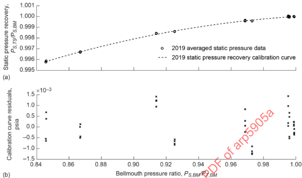
Figure 11 - Example of centerline static pressure calibration data
