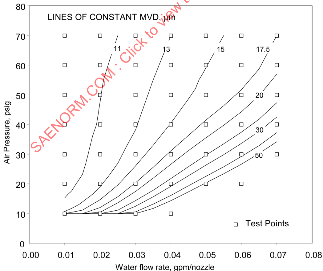
Figure 13 - Facility droplet size MVD calibration
