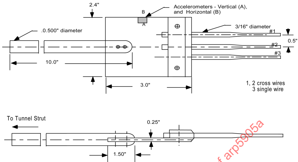
Figure 8 - Example of hot wire anemometer instrumentation probe
