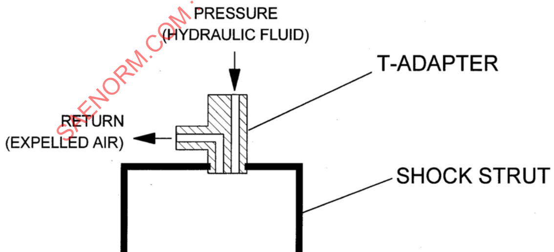
FIGURE 5 - TYPE III HYDRAULIC FLUID SERVICING
