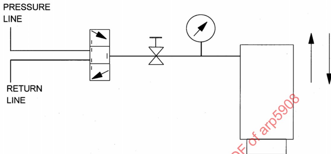
FIGURE 6 - TYPE IV HYDRAULIC FLUID SERVICING
