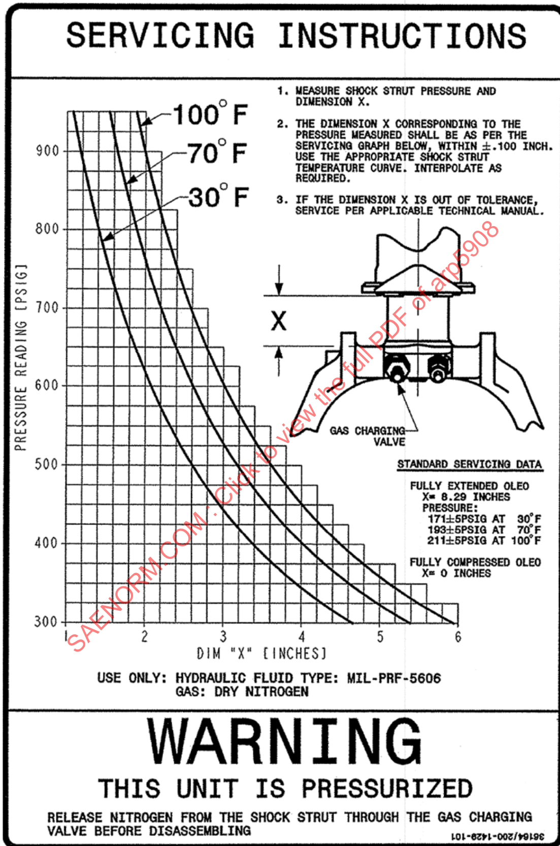
FIGURE 10 - SERVICING PLATE EXAMPLE – CHART FORMAT
