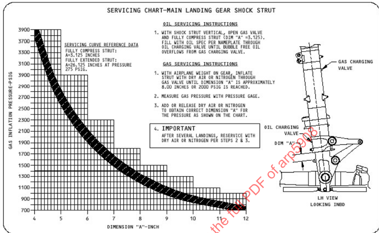
FIGURE 9 - SERVICING PLATE EXAMPLE – CHART FORMAT
