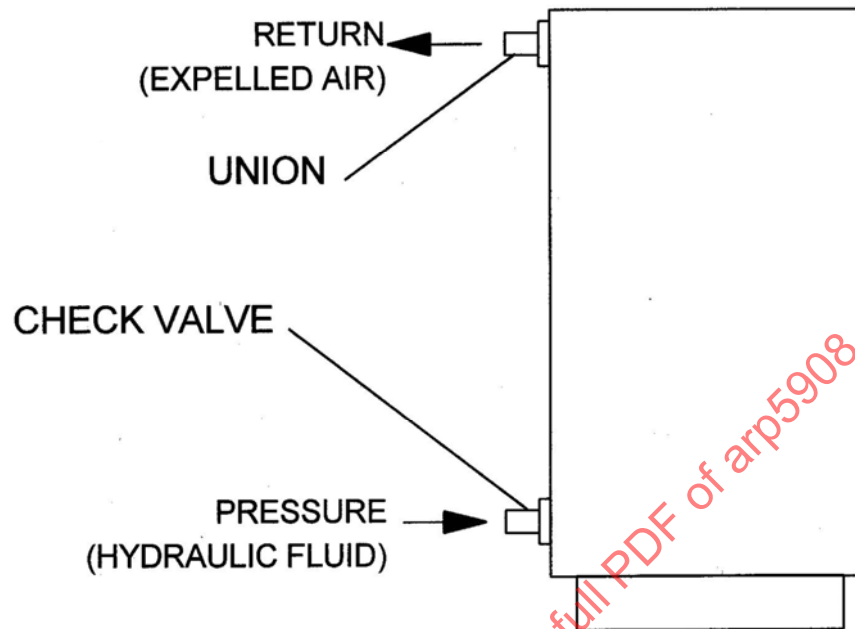
FIGURE 4 - TYPE II HYDRAULIC FLUID SERVICING
