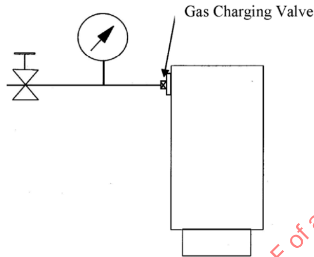
FIGURE 2 - LINE PRESSURIZED TO PREVENT PRESSURE LOSS
