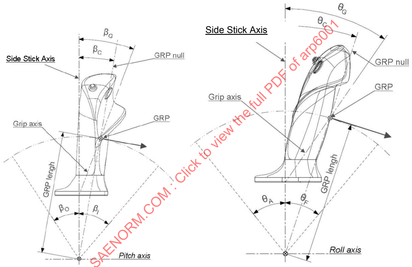
FIGURE 1 - SIDE STICK GEOMETRY DEFINITIONS AT MECHANICAL NULL
