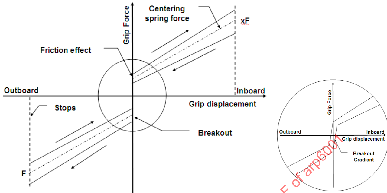
FIGURE 4 - NOTIONAL GRIP FORCE PROFILE IN ROLL
