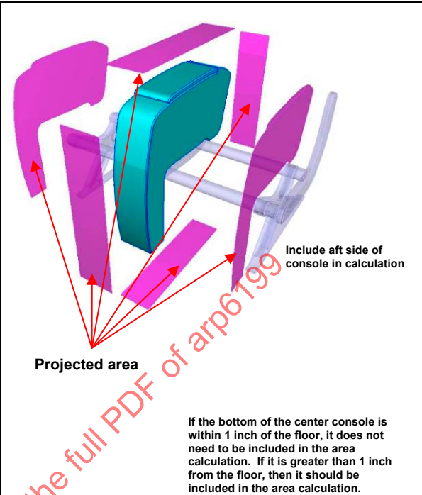
FIGURE 10 - CENTER CONSOLE AREA CALCULATION
