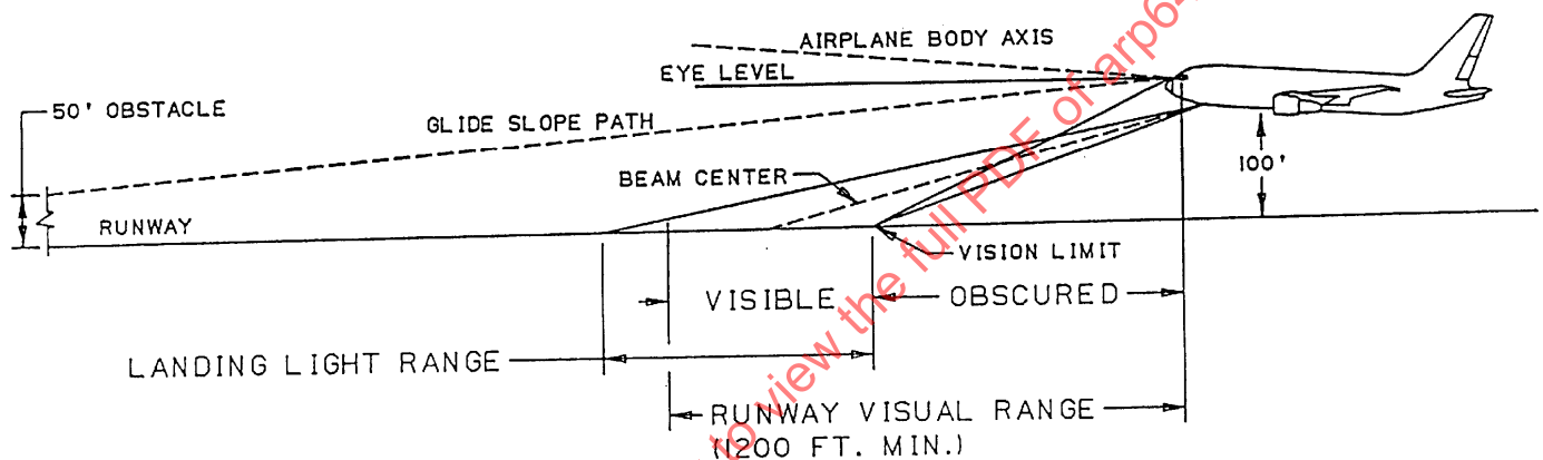
FIGURE 1 - LANDING LIGHT AT APPROACH ATTITUDE
