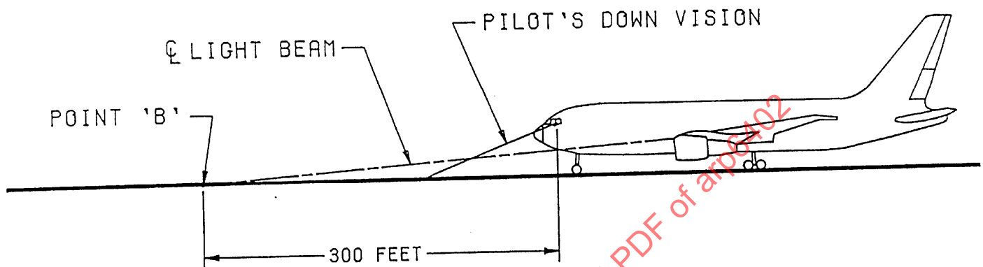
FIGURE 3 - LANDING LIGHT AT GROUND ROLL ATTITUDE
