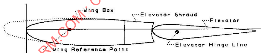
Wing-Flap Model
