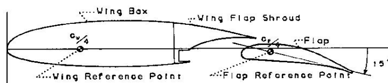
Figure B2 - Geometry of DHC-8 wing/flap and tailplane/elevator 2D models
