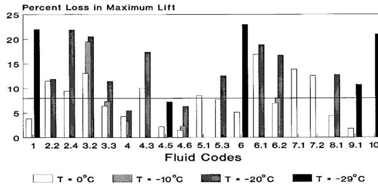
Figure B4 - Wing/flap model decrement in c_{lmax} , undiluted fluids, V_{rot} = 60 kts
