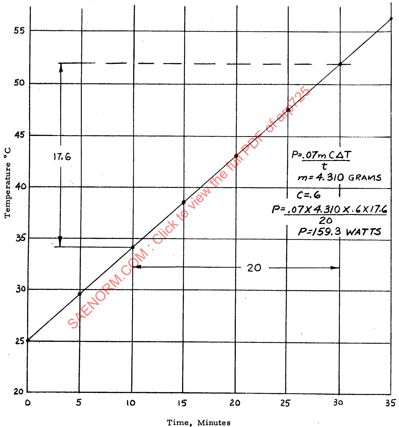
Figure 5. Typical Heat Rise Curve with Sample Calculation
