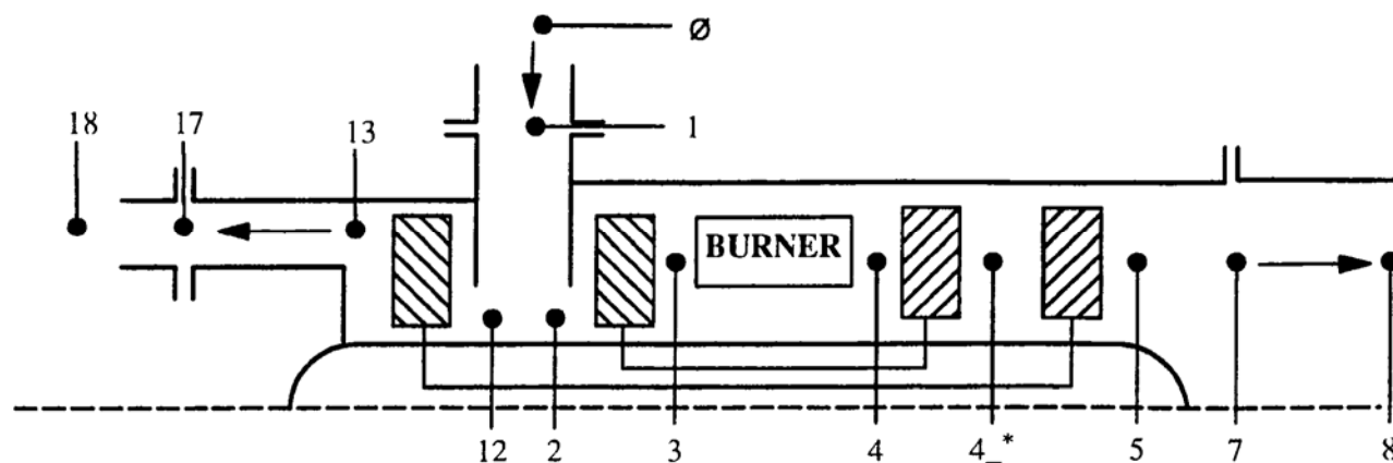
AUXILIARY POWER UNIT (Independent secondary compressor drive)
