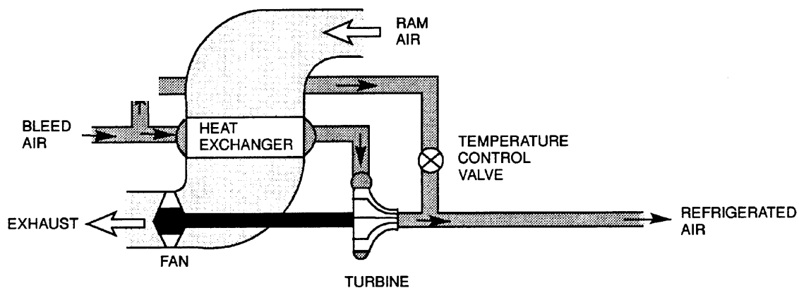
FIGURE 5A – SIMPLE CYCLE (TURBINE-FAN)
